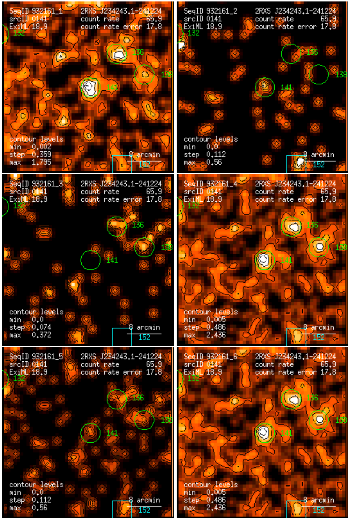
Figure 141: RASS 932161: detection 0141: band rate images, Gaussian filter: (1) PSPC channels 11 – 41, (2) 52 – 90, (3) 91 – 201, (4) 11 – 235, (5) 52 – 201, (6) 11 – 201. Broad band rates in counts/ks. Band rate contour levels in counts/ks/arcmin 2 .
