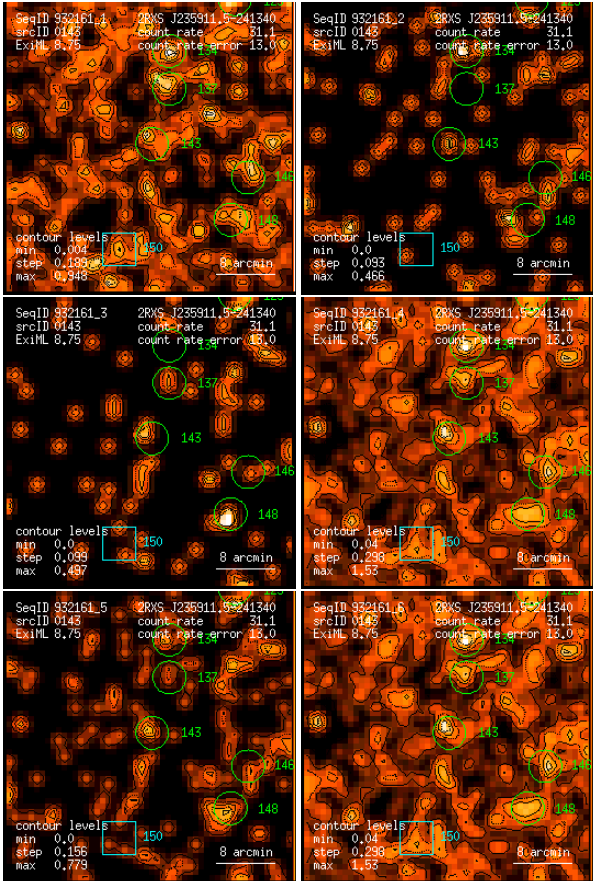
Figure 143: RASS 932161: detection 0143: band rate images, Gaussian filter: (1) PSPC channels 11 – 41, (2) 52 – 90, (3) 91 – 201, (4) 11 – 235, (5) 52 – 201, (6) 11 – 201. Broad band rates in counts/ks. Band rate contour levels in counts/ks/arcmin 2 .
