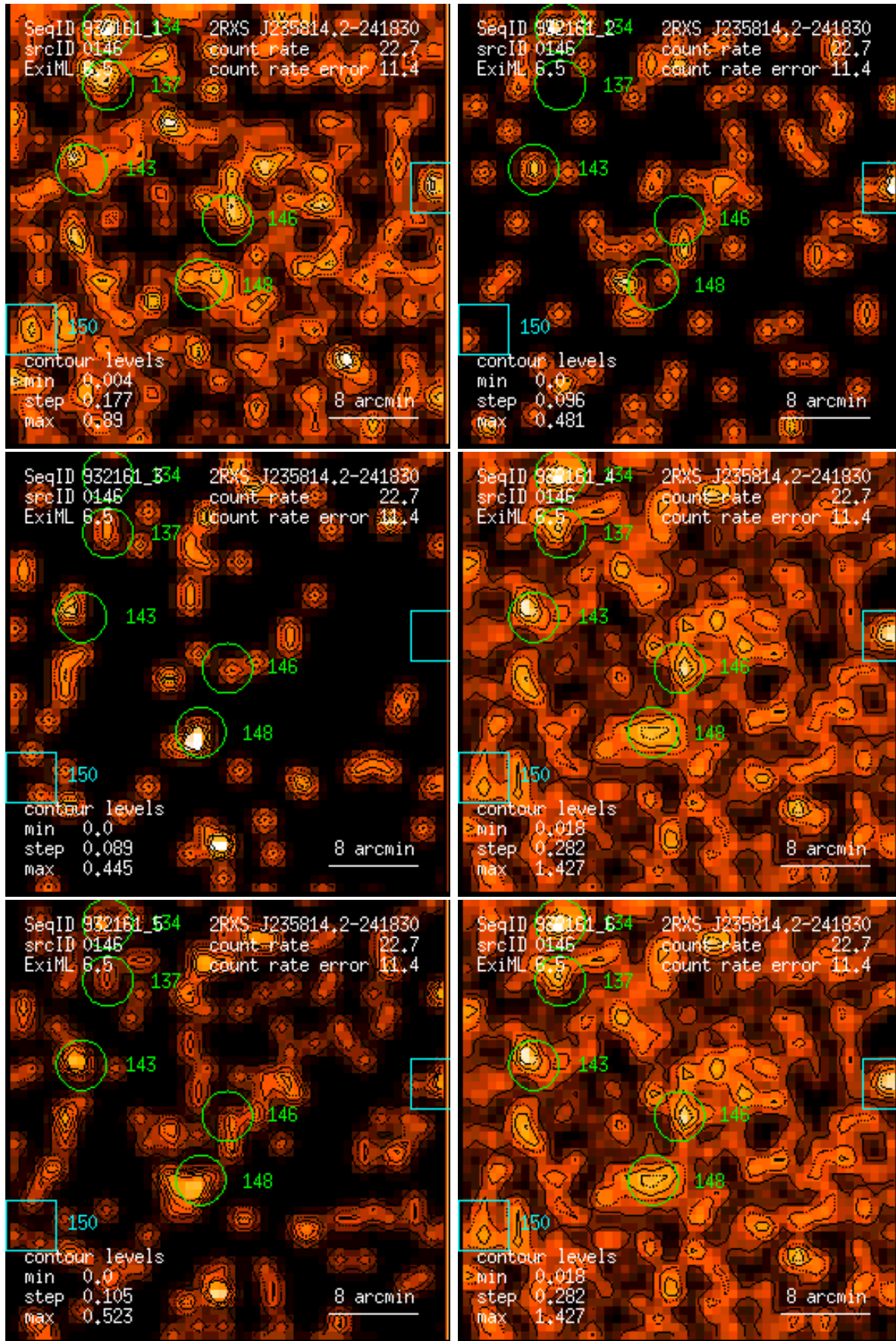
Figure 146: RASS 932161: detection 0146: band rate images, Gaussian filter: (1) PSPC channels 11 – 41, (2) 52 – 90, (3) 91 – 201, (4) 11 – 235, (5) 52 – 201, (6) 11 – 201. Broad band rates in counts/ks. Band rate contour levels in counts/ks/arcmin 2 .
