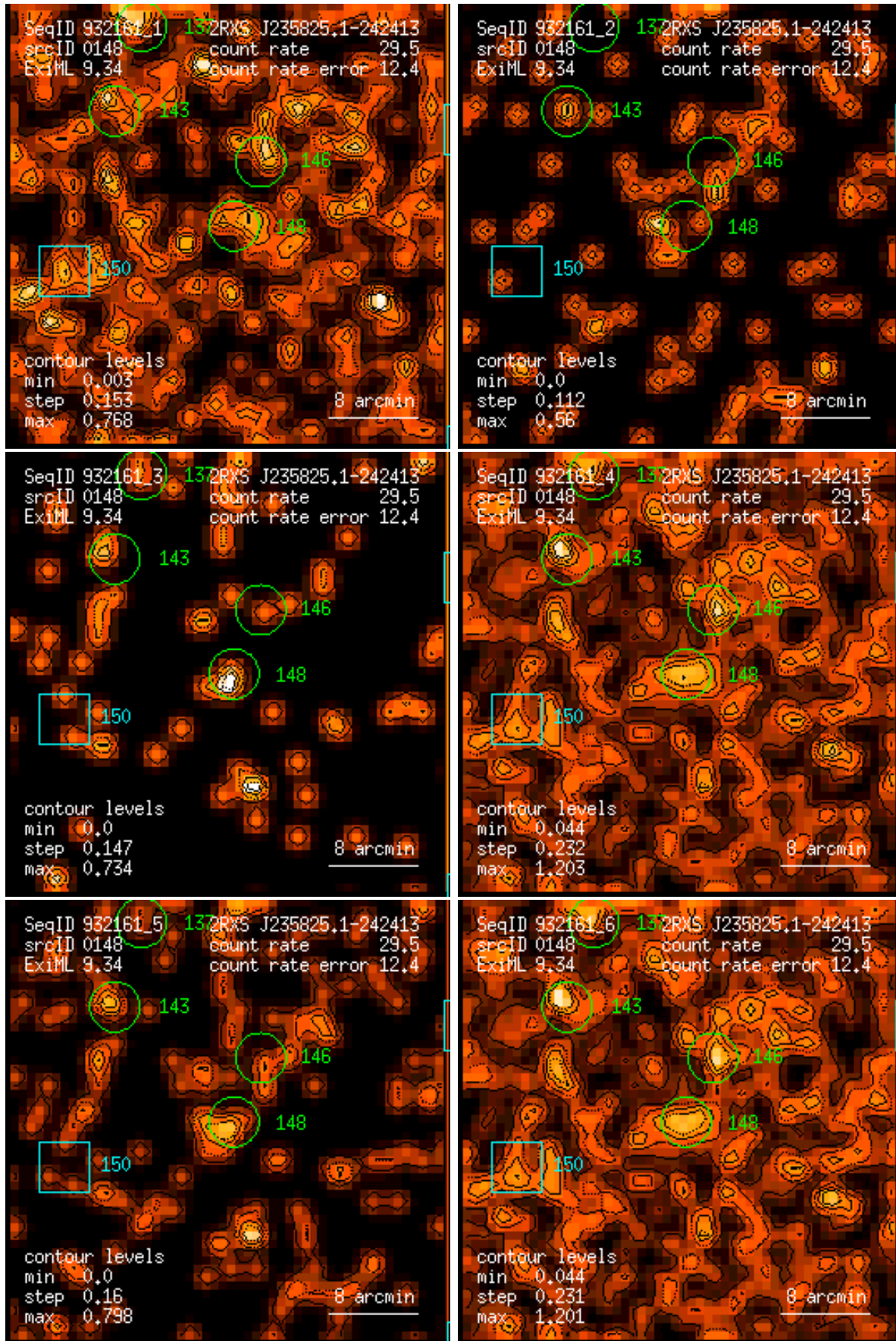
Figure 148: RASS 932161: detection 0148: band rate images, Gaussian filter: (1) PSPC channels 11 – 41, (2) 52 – 90, (3) 91 – 201, (4) 11 – 235, (5) 52 – 201, (6) 11 – 201. Broad band rates in counts/ks. Band rate contour levels in counts/ks/arcmin 2 .
