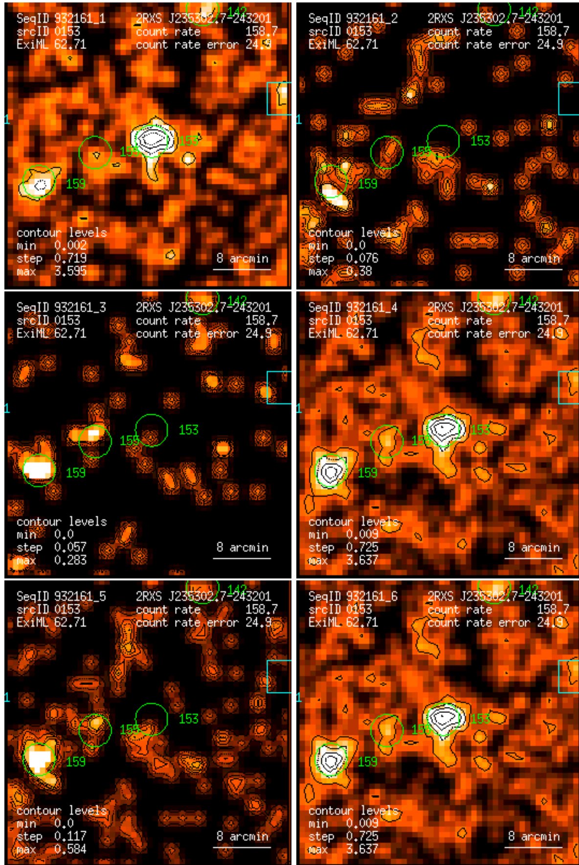
Figure 153: RASS 932161: detection 0153: band rate images, Gaussian filter: (1) PSPC channels 11 – 41, (2) 52 – 90, (3) 91 – 201, (4) 11 – 235, (5) 52 – 201, (6) 11 – 201. Broad band rates in counts/ks. Band rate contour levels in counts/ks/arcmin 2 .
