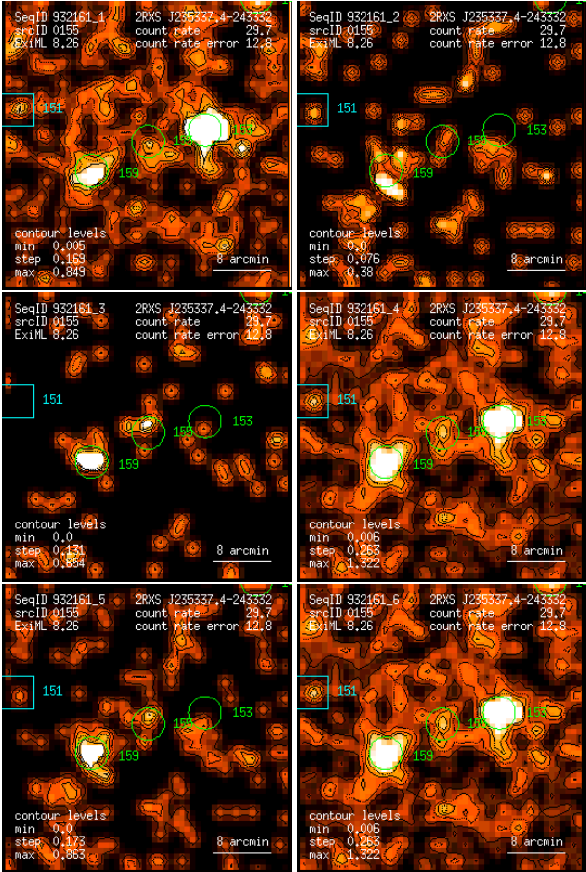
Figure 155: RASS 932161: detection 0155: band rate images, Gaussian filter: (1) PSPC channels 11 – 41, (2) 52 – 90, (3) 91 – 201, (4) 11 – 235, (5) 52 – 201, (6) 11 – 201. Broad band rates in counts/ks. Band rate contour levels in counts/ks/arcmin 2 .
