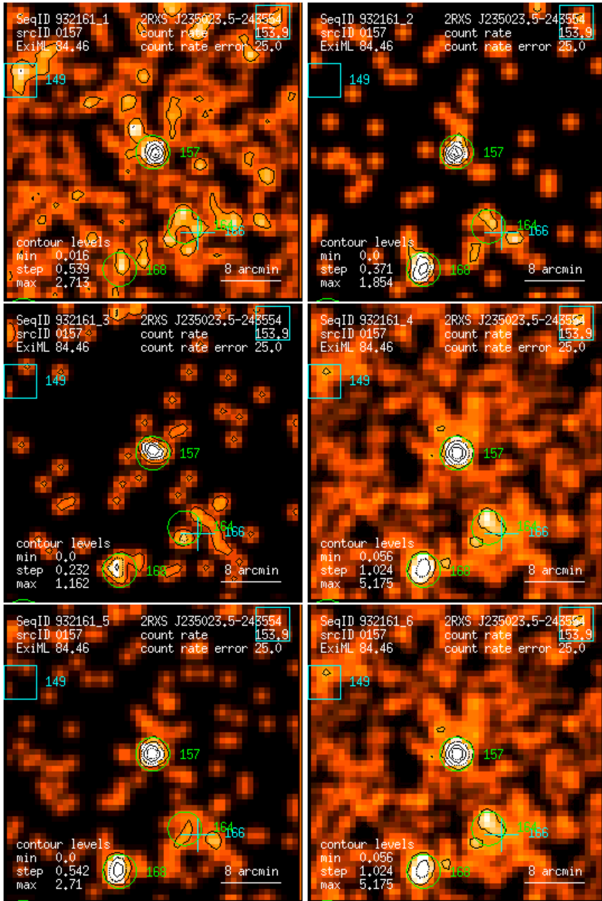
Figure 157: RASS 932161: detection 0157: band rate images, Gaussian filter: (1) PSPC channels 11 – 41, (2) 52 – 90, (3) 91 – 201, (4) 11 – 235, (5) 52 – 201, (6) 11 – 201. Broad band rates in counts/ks. Band rate contour levels in counts/ks/arcmin 2 .
