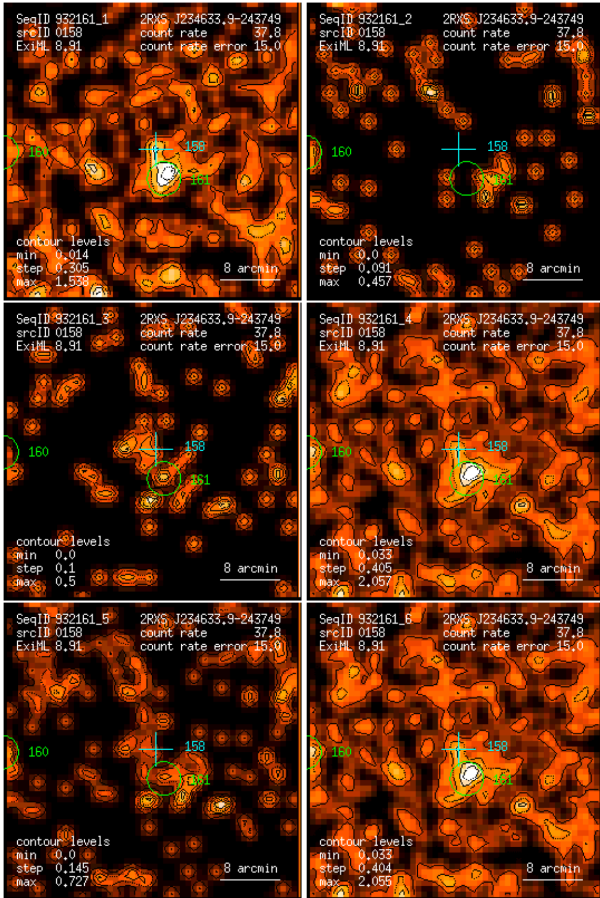
Figure 158: RASS 932161: detection 0158: band rate images, Gaussian filter: (1) PSPC channels 11 – 41, (2) 52 – 90, (3) 91 – 201, (4) 11 – 235, (5) 52 – 201, (6) 11 – 201. Broad band rates in counts/ks. Band rate contour levels in counts/ks/arcmin 2 .
