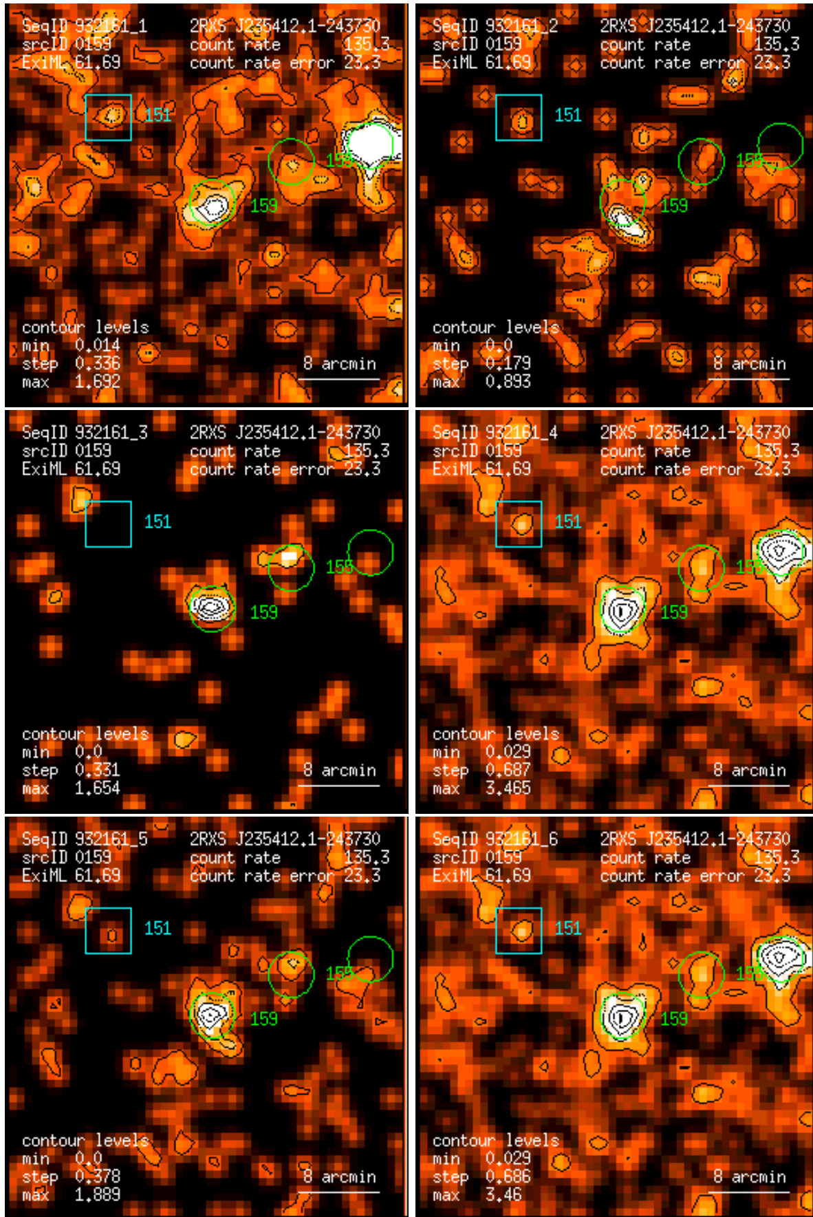
Figure 159: RASS 932161: detection 0159: band rate images, Gaussian filter: (1) PSPC channels 11 – 41, (2) 52 – 90, (3) 91 – 201, (4) 11 – 235, (5) 52 – 201, (6) 11 – 201. Broad band rates in counts/ks. Band rate contour levels in counts/ks/arcmin 2 .
