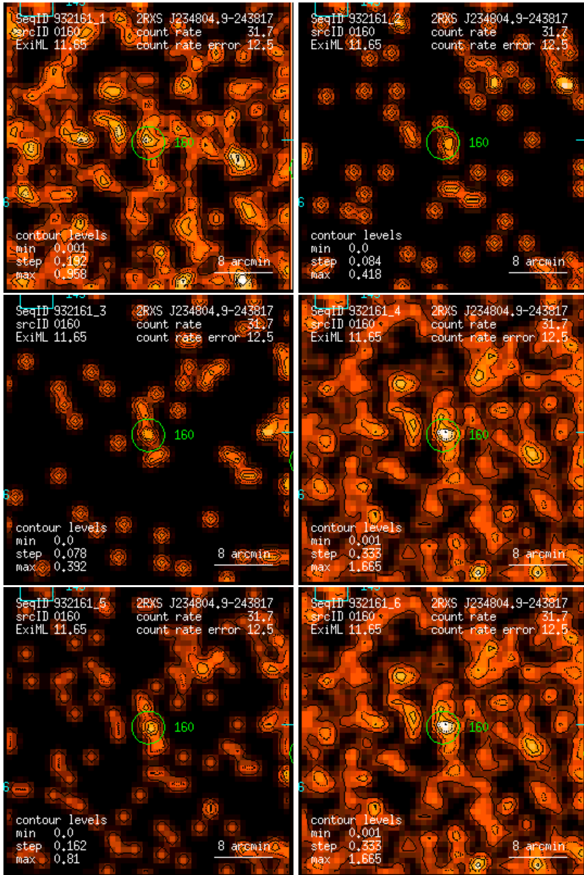
Figure 160: RASS 932161: detection 0160: band rate images, Gaussian filter: (1) PSPC channels 11 – 41, (2) 52 – 90, (3) 91 – 201, (4) 11 – 235, (5) 52 – 201, (6) 11 – 201. Broad band rates in counts/ks. Band rate contour levels in counts/ks/arcmin 2 .
