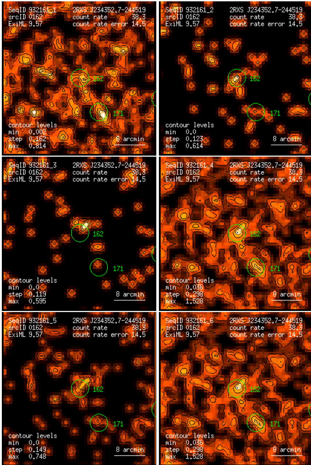
Figure 162: RASS 932161: detection 0162: band rate images, Gaussian filter: (1) PSPC channels 11 – 41, (2) 52 – 90, (3) 91 – 201, (4) 11 – 235, (5) 52 – 201, (6) 11 – 201. Broad band rates in counts/ks. Band rate contour levels in counts/ks/arcmin 2 .
