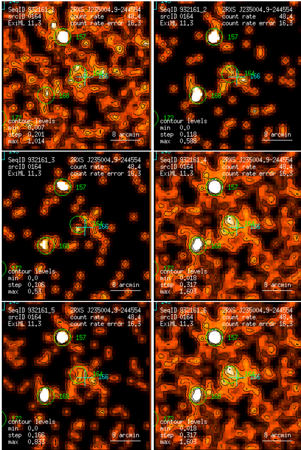
Figure 164: RASS 932161: detection 0164: band rate images, Gaussian filter: (1) PSPC channels 11 – 41, (2) 52 – 90, (3) 91 – 201, (4) 11 – 235, (5) 52 – 201, (6) 11 – 201. Broad band rates in counts/ks. Band rate contour levels in counts/ks/arcmin 2 .
