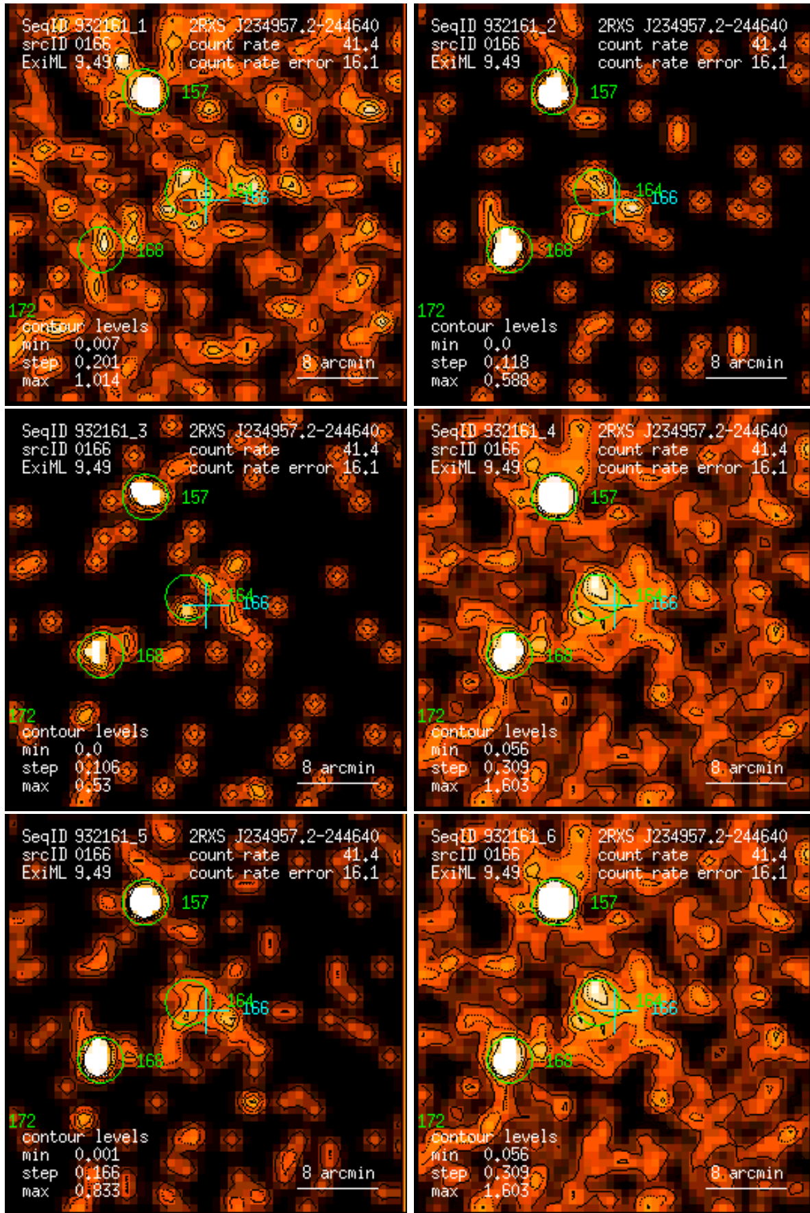
Figure 166: RASS 932161: detection 0166: band rate images, Gaussian filter: (1) PSPC channels 11 – 41, (2) 52 – 90, (3) 91 – 201, (4) 11 – 235, (5) 52 – 201, (6) 11 – 201. Broad band rates in counts/ks. Band rate contour levels in counts/ks/arcmin 2 .
