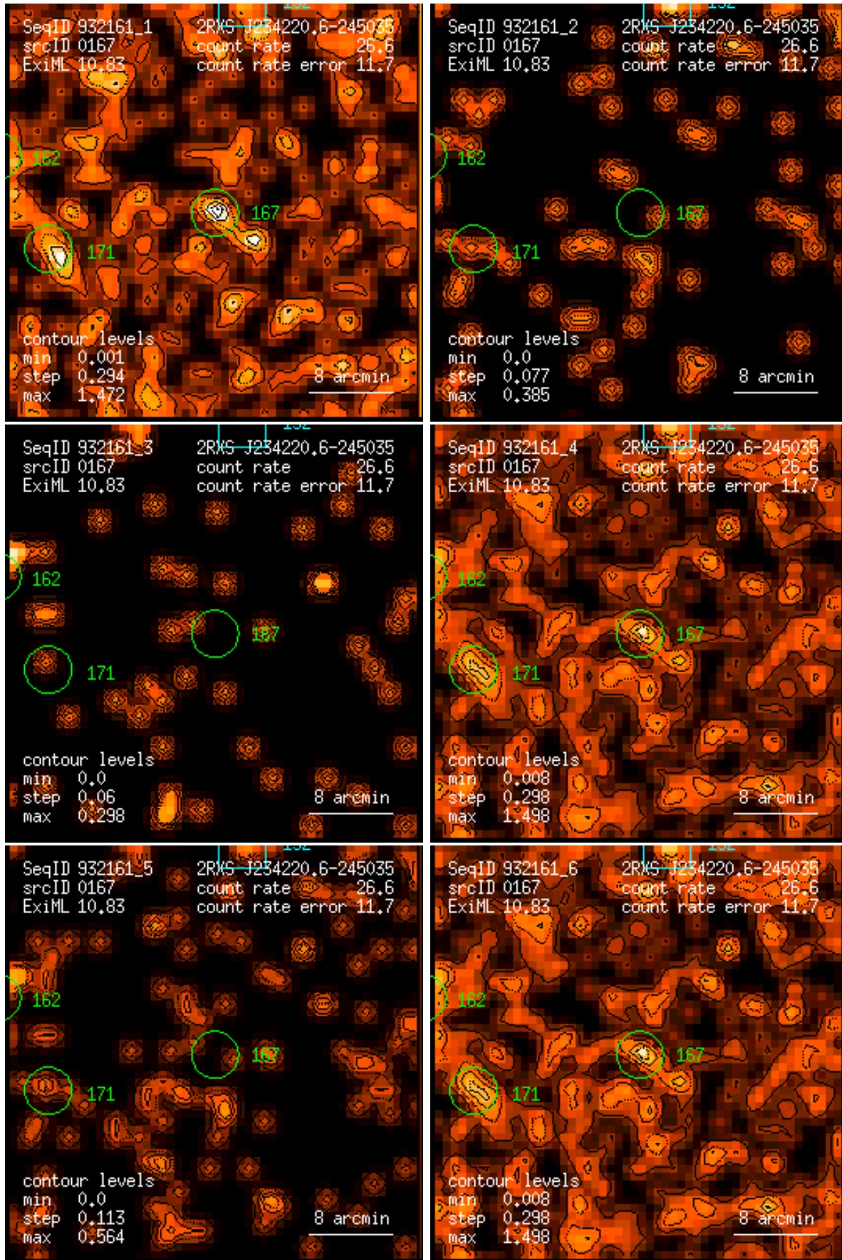
Figure 167: RASS 932161: detection 0167: band rate images, Gaussian filter: (1) PSPC channels 11 – 41, (2) 52 – 90, (3) 91 – 201, (4) 11 – 235, (5) 52 – 201, (6) 11 – 201. Broad band rates in counts/ks. Band rate contour levels in counts/ks/arcmin 2 .
