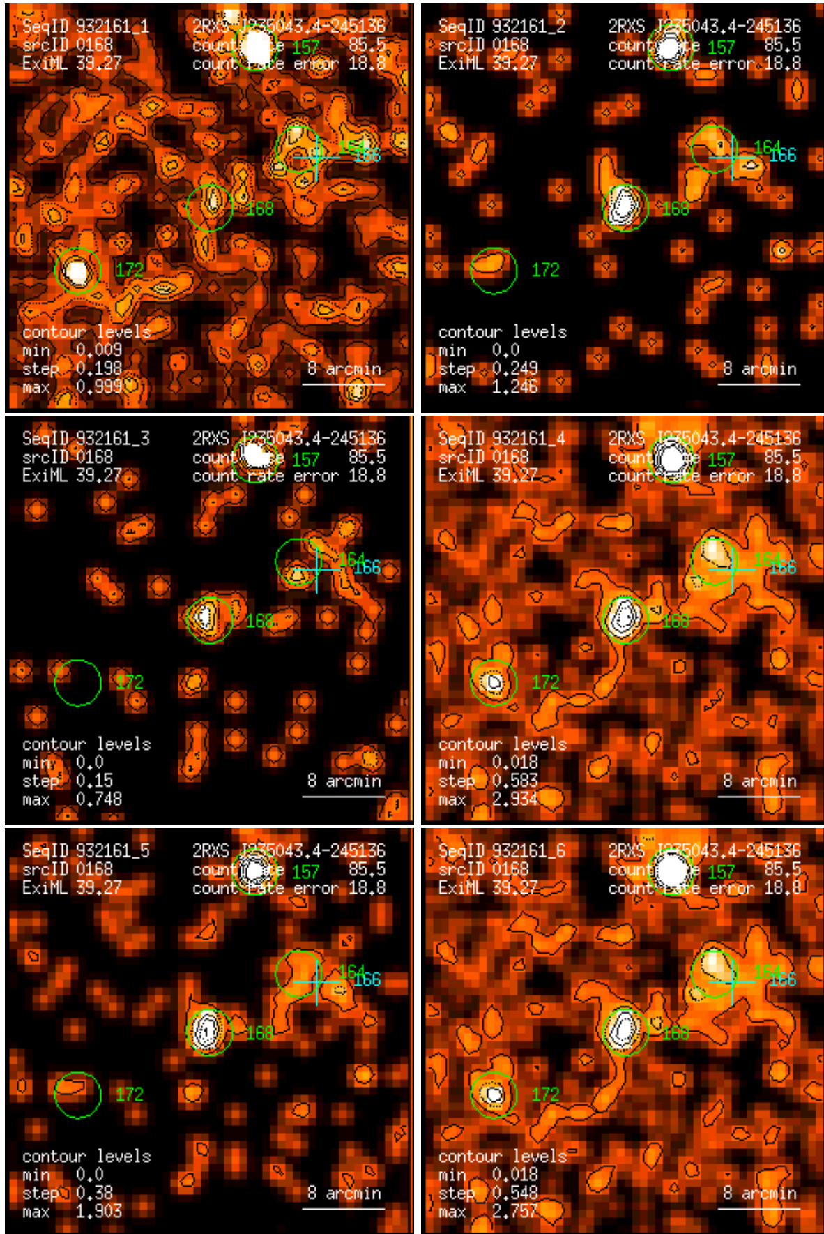
Figure 168: RASS 932161: detection 0168: band rate images, Gaussian filter: (1) PSPC channels 11 – 41, (2) 52 – 90, (3) 91 – 201, (4) 11 – 235, (5) 52 – 201, (6) 11 – 201. Broad band rates in counts/ks. Band rate contour levels in counts/ks/arcmin 2 .
