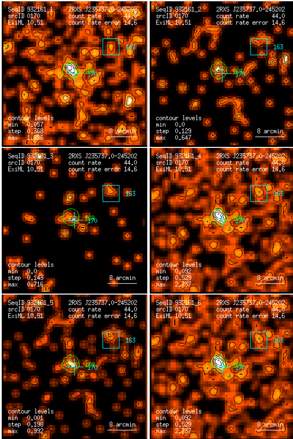
Figure 170: RASS 932161: detection 0170: band rate images, Gaussian filter: (1) PSPC channels 11 – 41, (2) 52 – 90, (3) 91 – 201, (4) 11 – 235, (5) 52 – 201, (6) 11 – 201. Broad band rates in counts/ks. Band rate contour levels in counts/ks/arcmin 2 .
