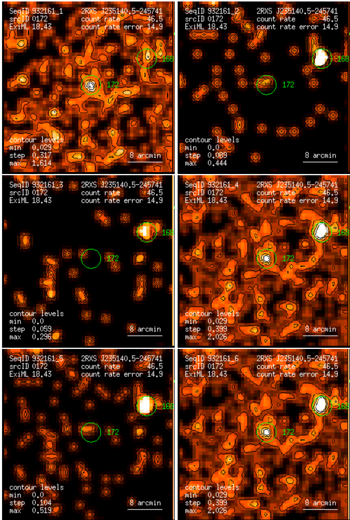
Figure 172: RASS 932161: detection 0172: band rate images, Gaussian filter: (1) PSPC channels 11 – 41, (2) 52 – 90, (3) 91 – 201, (4) 11 – 235, (5) 52 – 201, (6) 11 – 201. Broad band rates in counts/ks. Band rate contour levels in counts/ks/arcmin 2 .
