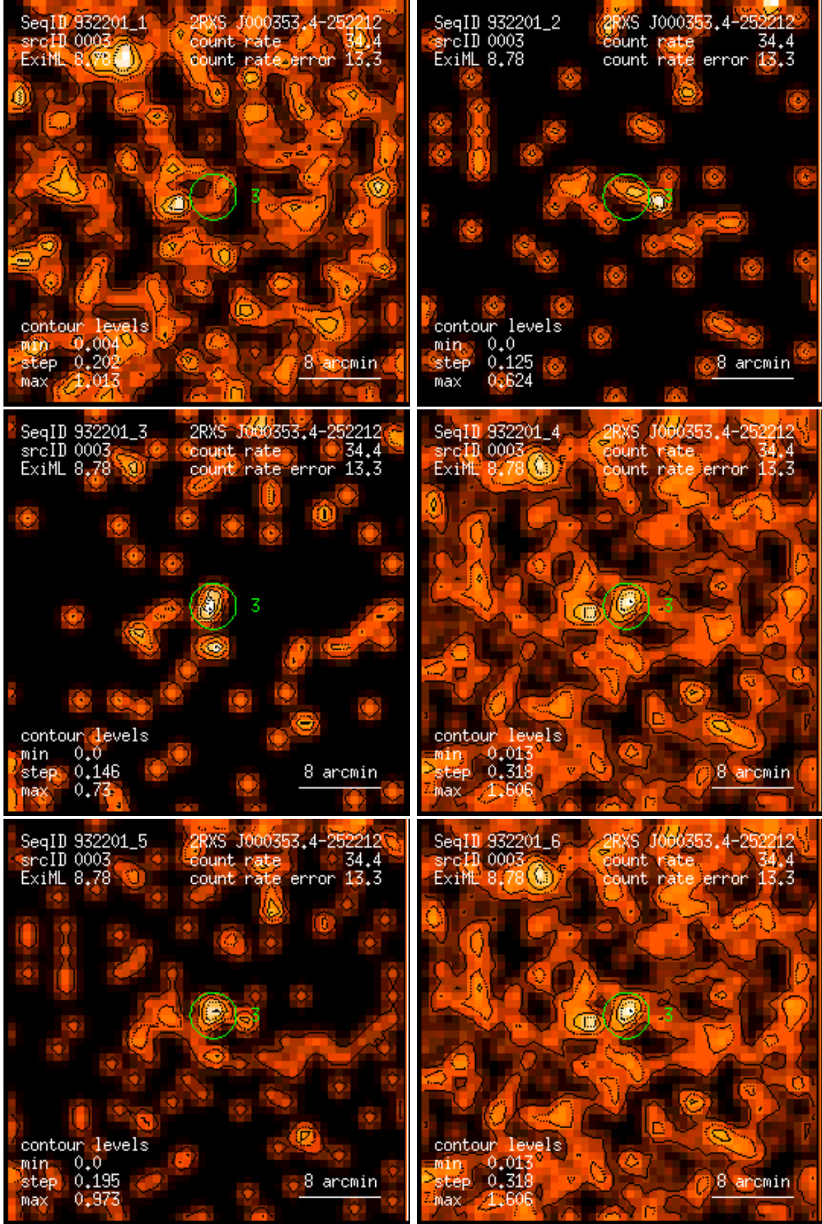
Figure 3: RASS 932201: detection 0003: band rate images, Gaussian filter: (1) PSPC channels 11 – 41, (2) 52 – 90, (3) 91 – 201, (4) 11 – 235, (5) 52 – 201, (6) 11 – 201. Broad band rates in counts/ks. Band rate contour levels in counts/ks/arcmin 2 .
