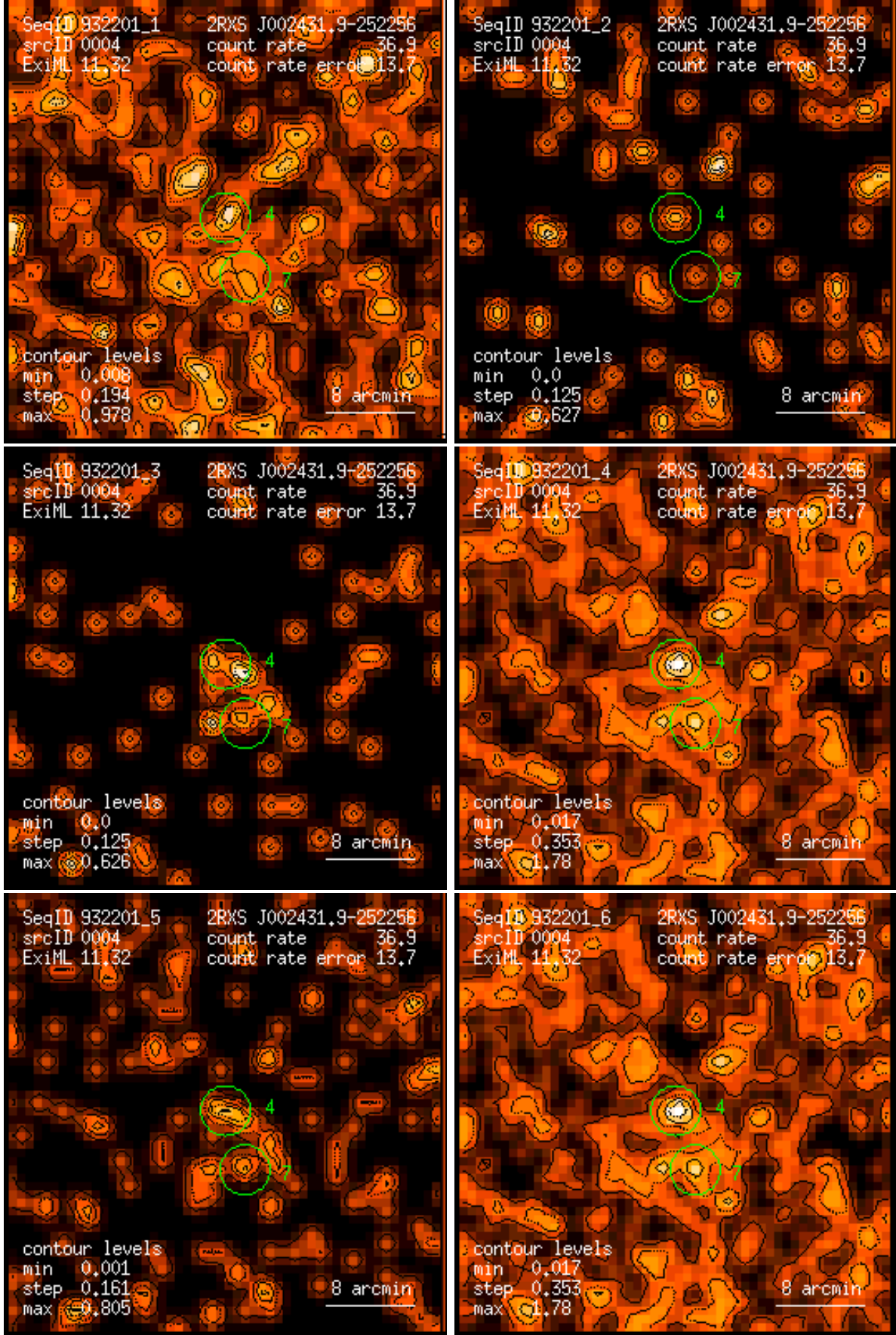
Figure 4: RASS 932201: detection 0004: band rate images, Gaussian filter: (1) PSPC channels 11 – 41, (2) 52 – 90, (3) 91 – 201, (4) 11 – 235, (5) 52 – 201, (6) 11 – 201. Broad band rates in counts/ks. Band rate contour levels in counts/ks/arcmin 2 .
