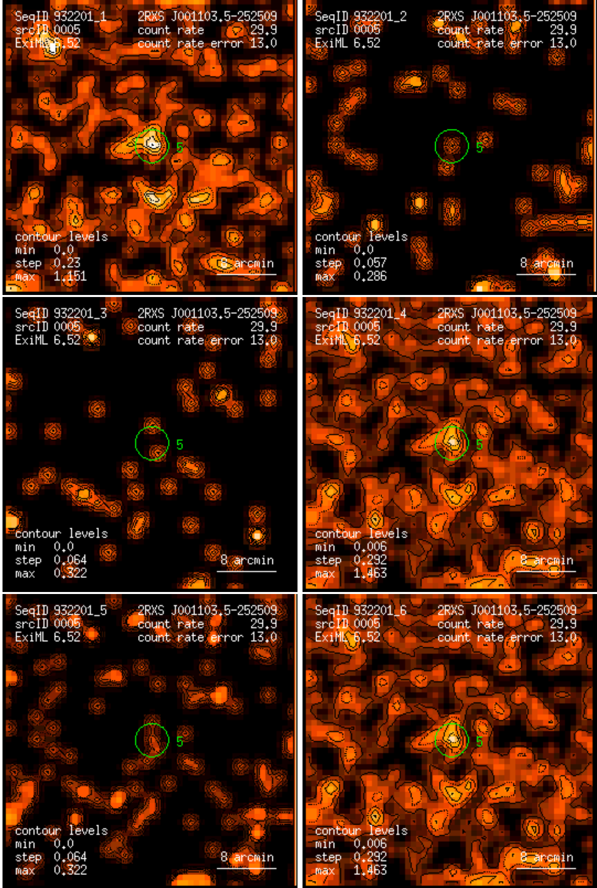
Figure 5: RASS 932201: detection 0005: band rate images, Gaussian filter: (1) PSPC channels 11 – 41, (2) 52 – 90, (3) 91 – 201, (4) 11 – 235, (5) 52 – 201, (6) 11 – 201. Broad band rates in counts/ks. Band rate contour levels in counts/ks/arcmin 2 .
