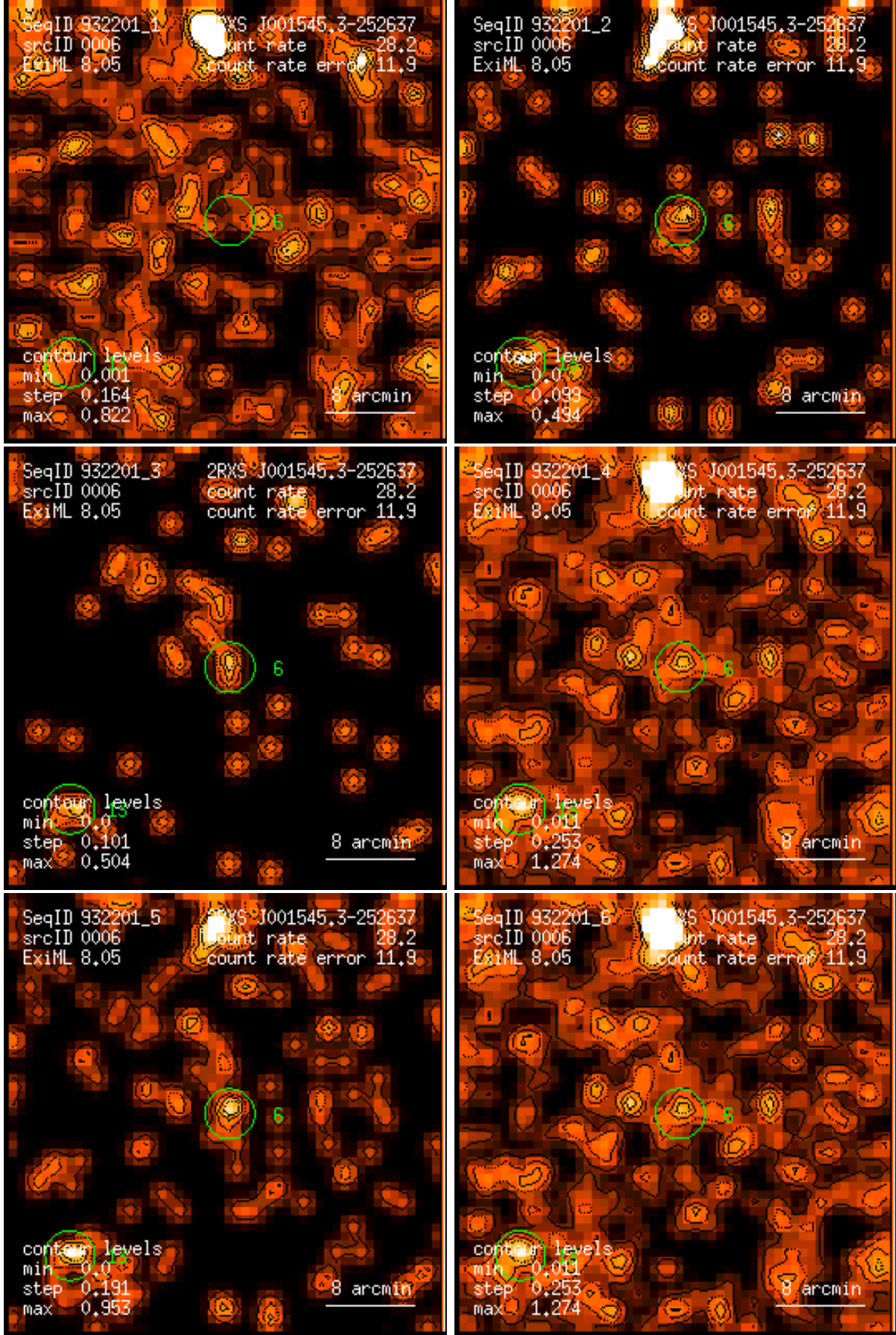
Figure 6: RASS 932201: detection 0006: band rate images, Gaussian filter: (1) PSPC channels 11 – 41, (2) 52 – 90, (3) 91 – 201, (4) 11 – 235, (5) 52 – 201, (6) 11 – 201. Broad band rates in counts/ks. Band rate contour levels in counts/ks/arcmin 2 .
