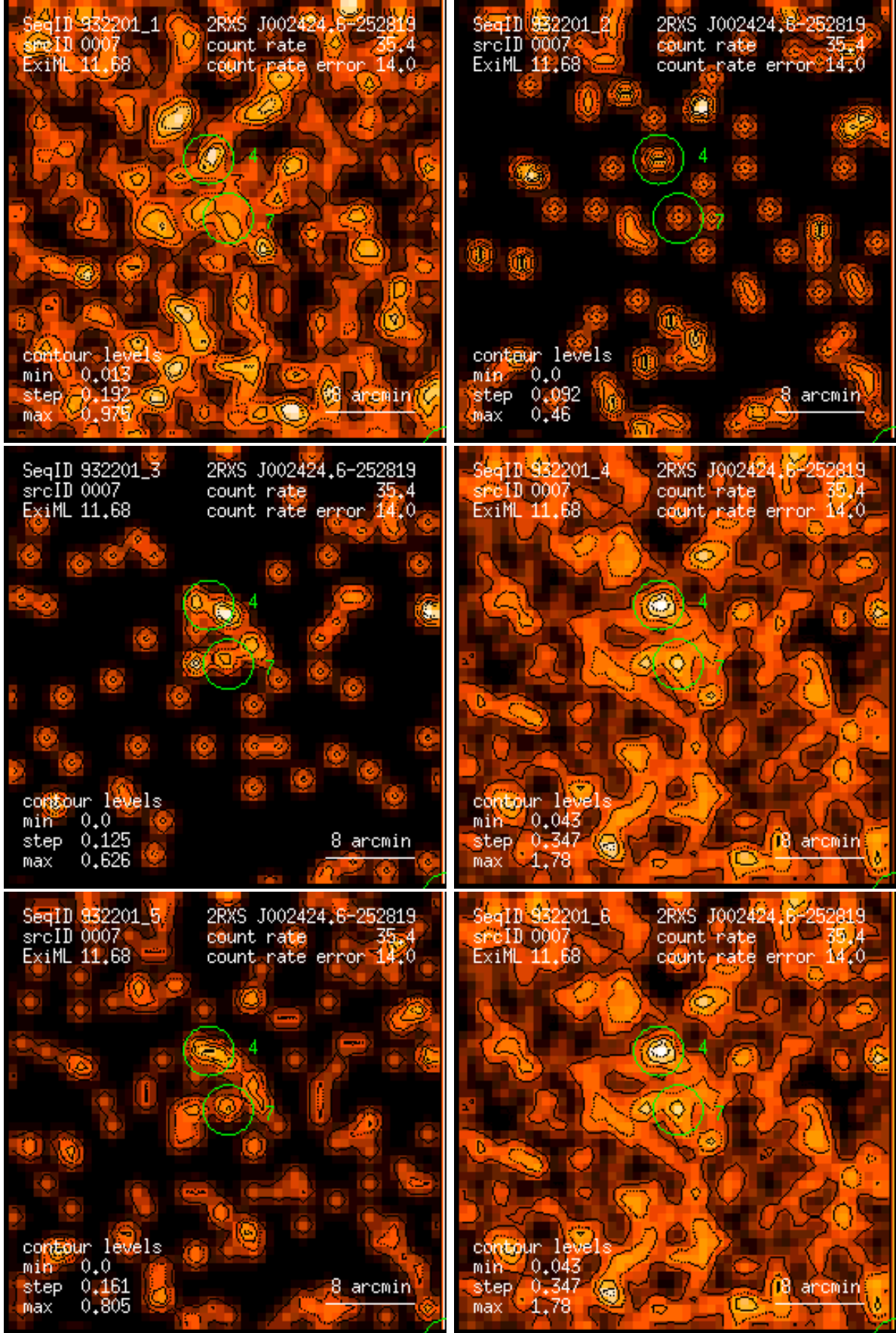
Figure 7: RASS 932201: detection 0007: band rate images, Gaussian filter: (1) PSPC channels 11 – 41, (2) 52 – 90, (3) 91 – 201, (4) 11 – 235, (5) 52 – 201, (6) 11 – 201. Broad band rates in counts/ks. Band rate contour levels in counts/ks/arcmin 2 .
