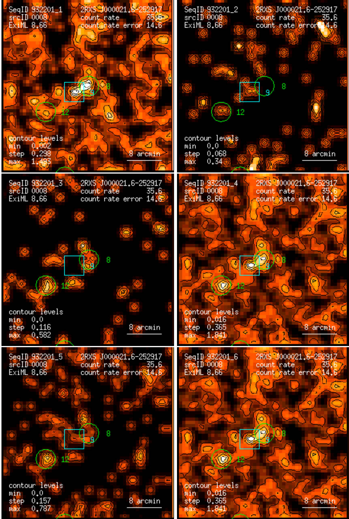
Figure 8: RASS 932201: detection 0008: band rate images, Gaussian filter: (1) PSPC channels 11 – 41, (2) 52 – 90, (3) 91 – 201, (4) 11 – 235, (5) 52 – 201, (6) 11 – 201. Broad band rates in counts/ks. Band rate contour levels in counts/ks/arcmin 2 .
