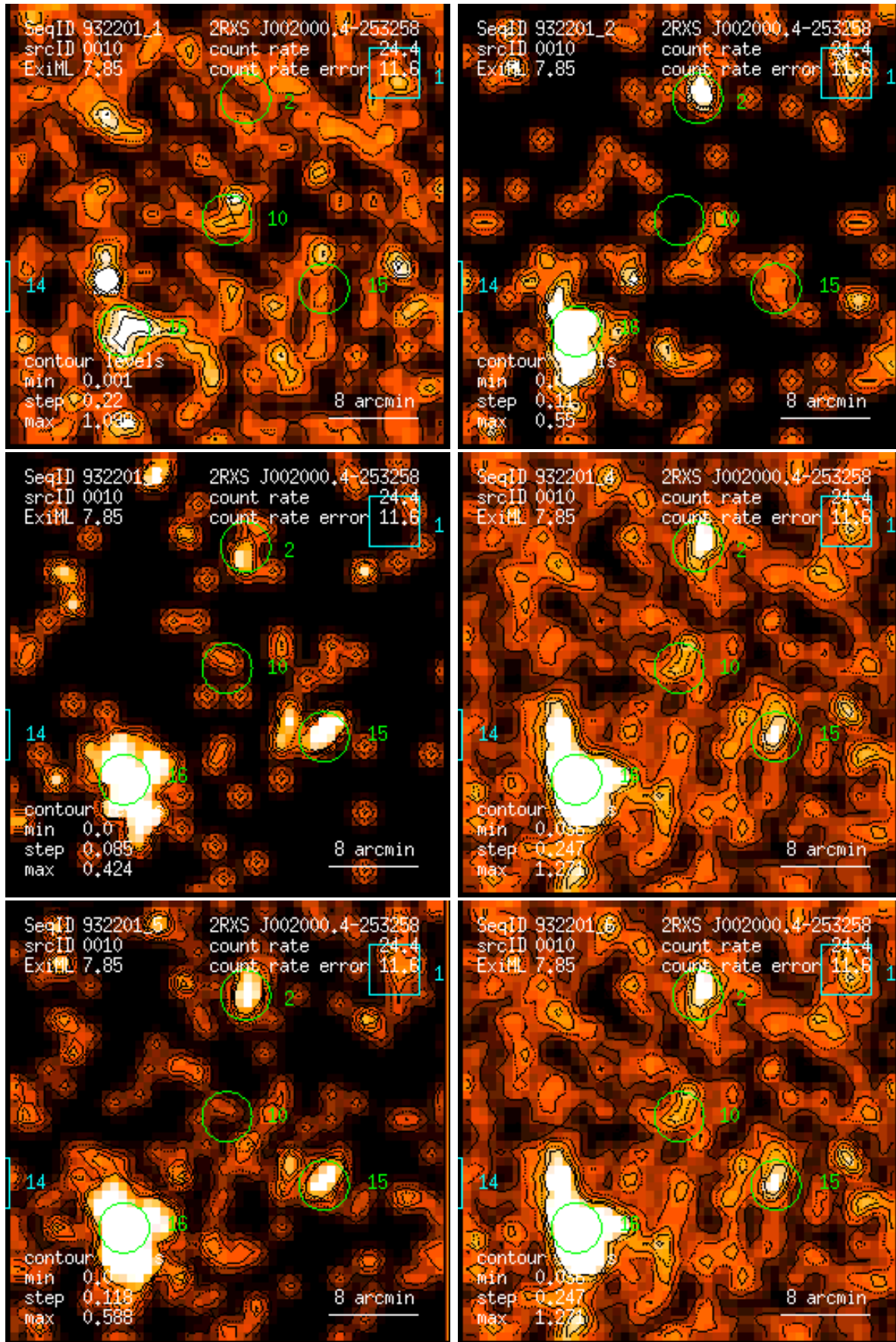
Figure 10: RASS 932201: detection 0010: band rate images, Gaussian filter: (1) PSPC channels 11 – 41, (2) 52 – 90, (3) 91 – 201, (4) 11 – 235, (5) 52 – 201, (6) 11 – 201. Broad band rates in counts/ks. Band rate contour levels in counts/ks/arcmin 2 .
