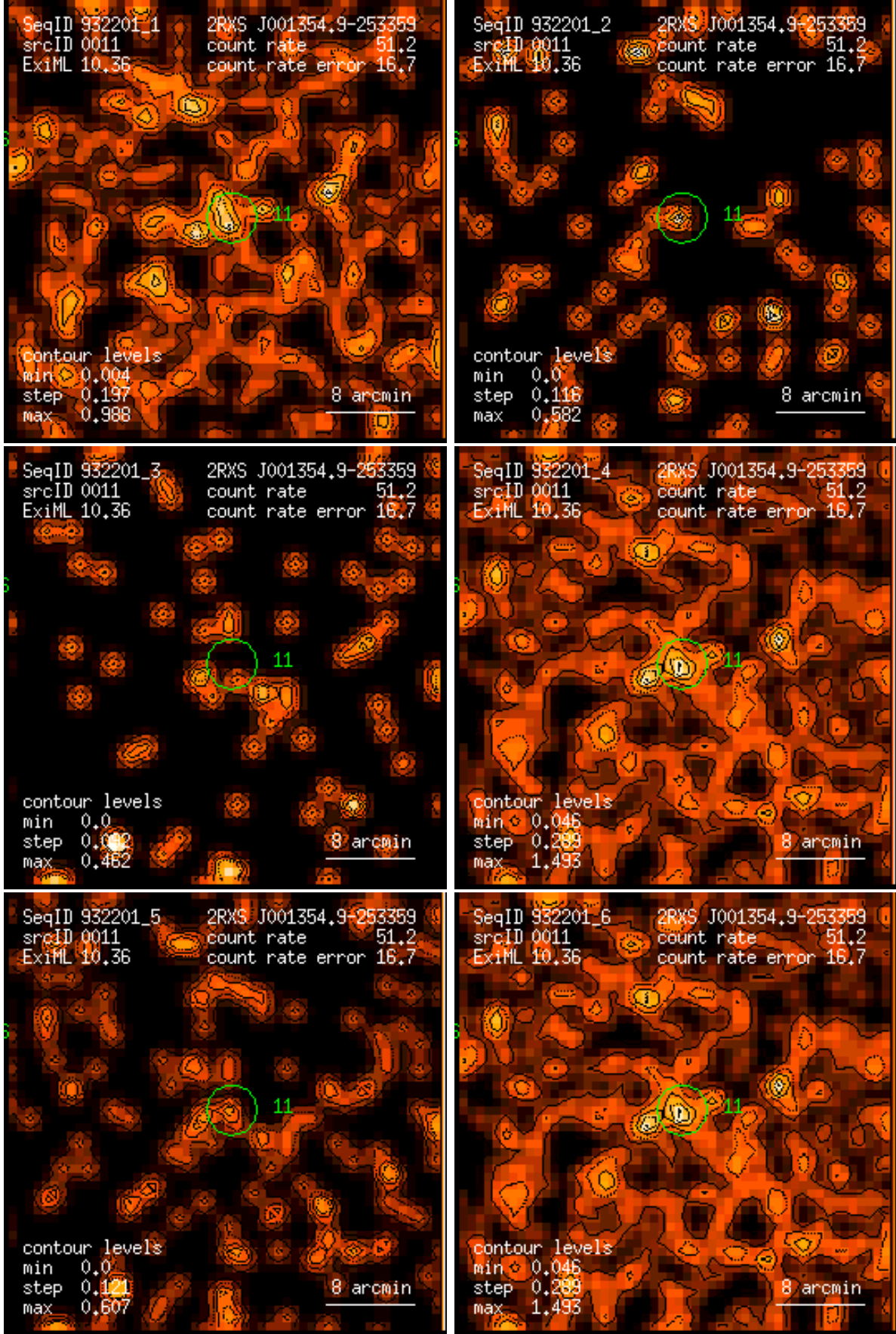
Figure 11: RASS 932201: detection 0011: band rate images, Gaussian filter: (1) PSPC channels 11 – 41, (2) 52 – 90, (3) 91 – 201, (4) 11 – 235, (5) 52 – 201, (6) 11 – 201. Broad band rates in counts/ks. Band rate contour levels in counts/ks/arcmin 2 .
