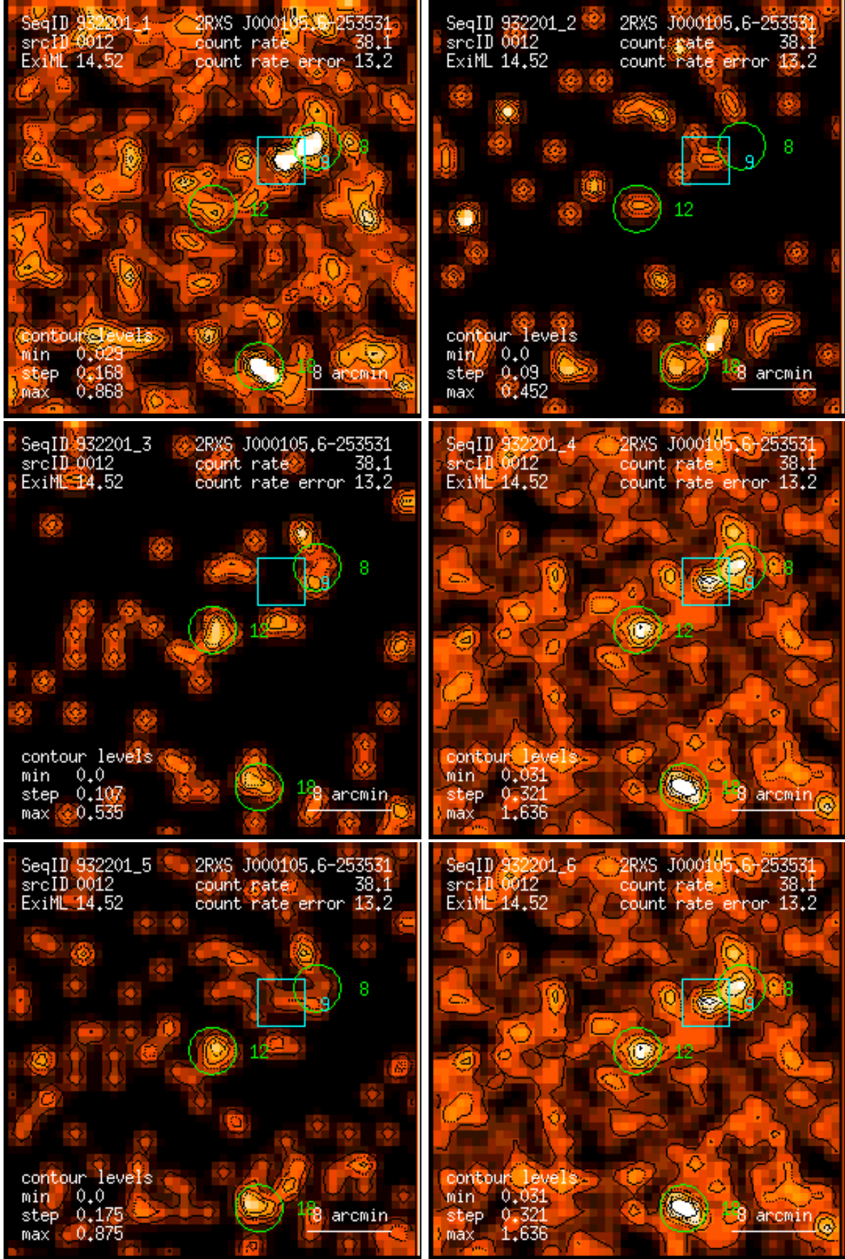
Figure 12: RASS 932201: detection 0012: band rate images, Gaussian filter: (1) PSPC channels 11 – 41, (2) 52 – 90, (3) 91 – 201, (4) 11 – 235, (5) 52 – 201, (6) 11 – 201. Broad band rates in counts/ks. Band rate contour levels in counts/ks/arcmin 2 .
