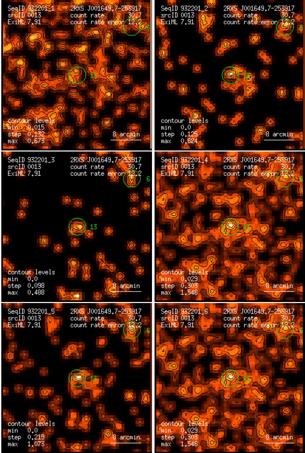
Figure 13: RASS 932201: detection 0013: band rate images, Gaussian filter: (1) PSPC channels 11 – 41, (2) 52 – 90, (3) 91 – 201, (4) 11 – 235, (5) 52 – 201, (6) 11 – 201. Broad band rates in counts/ks. Band rate contour levels in counts/ks/arcmin 2 .
