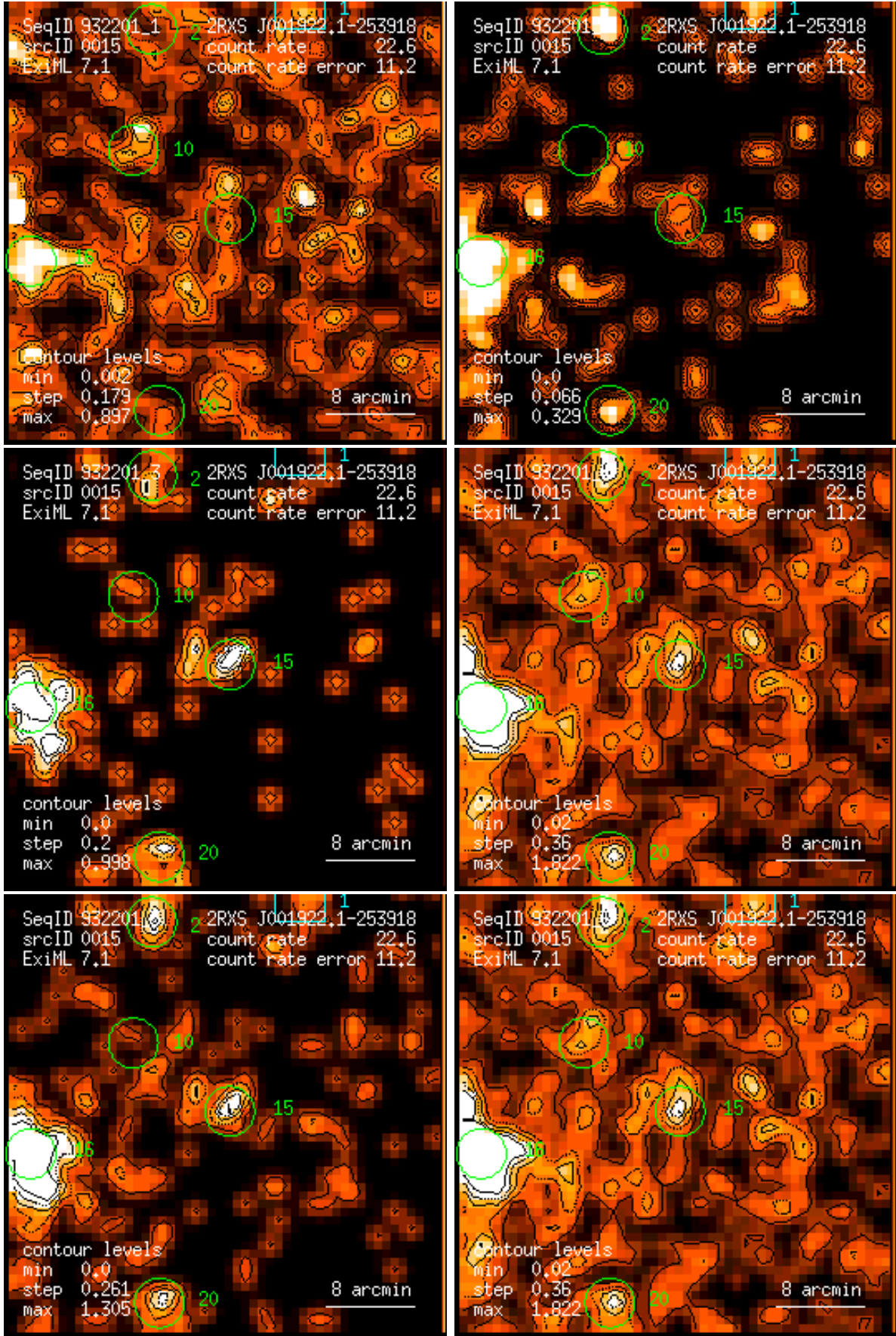
Figure 15: RASS 932201: detection 0015: band rate images, Gaussian filter: (1) PSPC channels 11 – 41, (2) 52 – 90, (3) 91 – 201, (4) 11 – 235, (5) 52 – 201, (6) 11 – 201. Broad band rates in counts/ks. Band rate contour levels in counts/ks/arcmin 2 .
