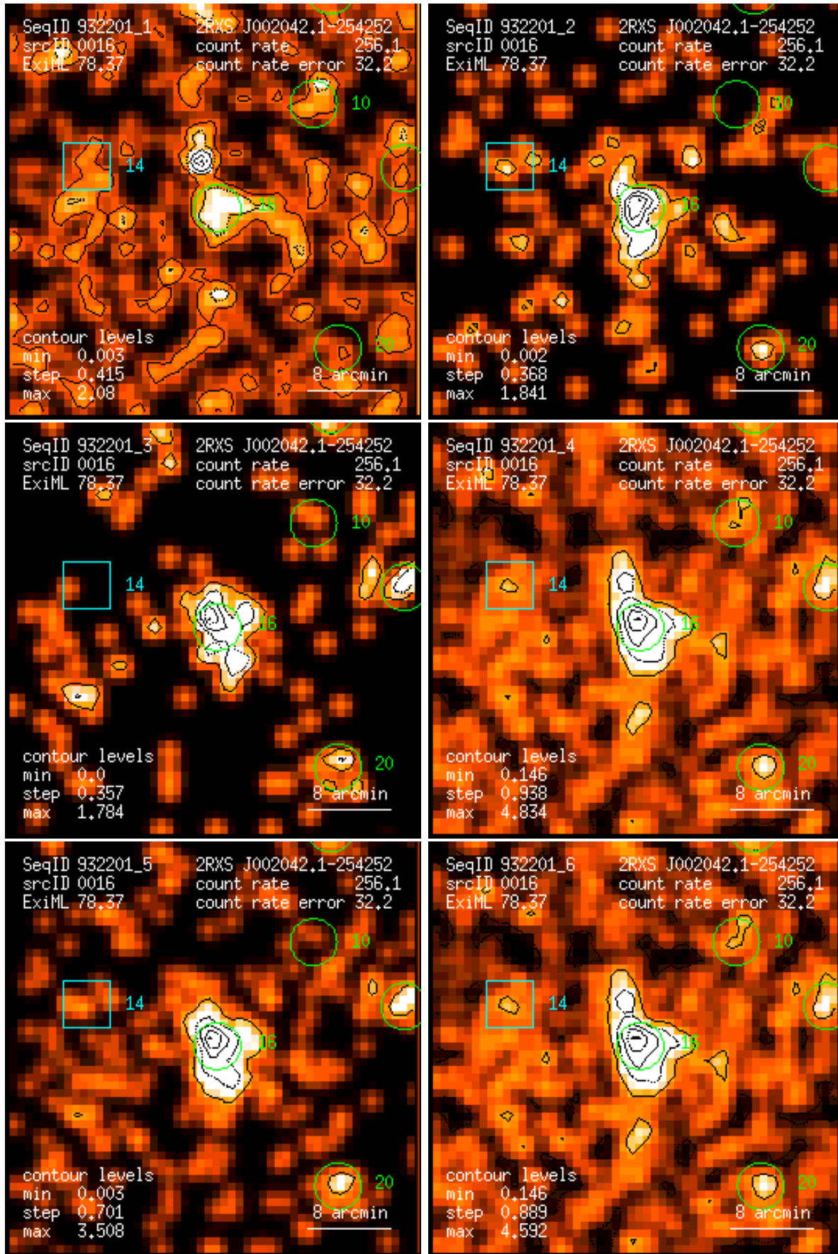
Figure 16: RASS 932201: detection 0016: band rate images, Gaussian filter: (1) PSPC channels 11 – 41, (2) 52 – 90, (3) 91 – 201, (4) 11 – 235, (5) 52 – 201, (6) 11 – 201. Broad band rates in counts/ks. Band rate contour levels in counts/ks/arcmin 2 .
