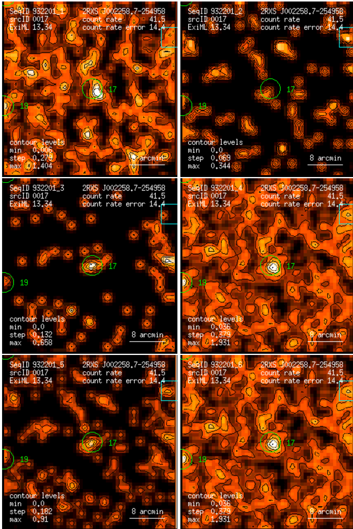
Figure 17: RASS 932201: detection 0017: band rate images, Gaussian filter: (1) PSPC channels 11 – 41, (2) 52 – 90, (3) 91 – 201, (4) 11 – 235, (5) 52 – 201, (6) 11 – 201. Broad band rates in counts/ks. Band rate contour levels in counts/ks/arcmin 2 .
