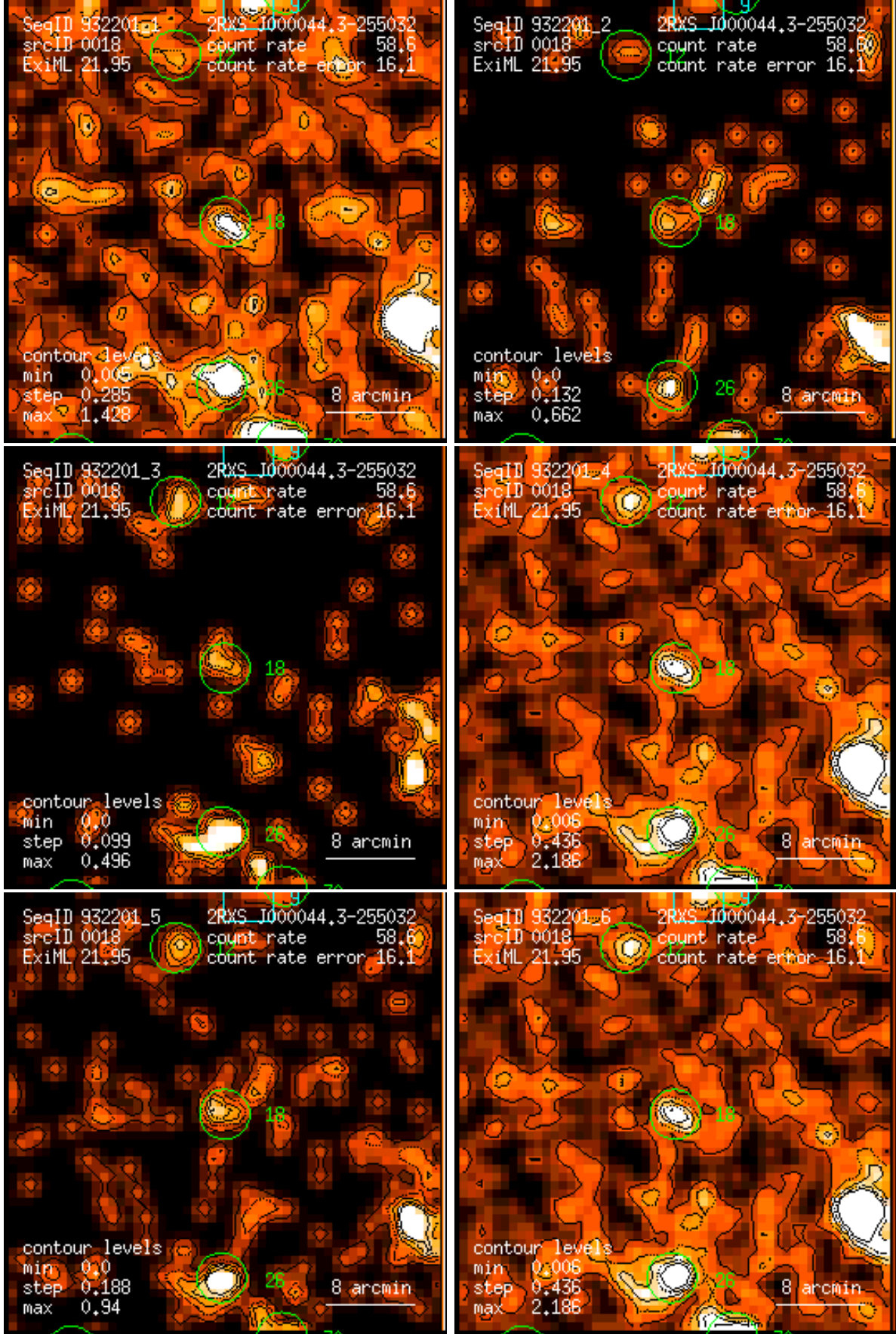
Figure 18: RASS 932201: detection 0018: band rate images, Gaussian filter: (1) PSPC channels 11 – 41, (2) 52 – 90, (3) 91 – 201, (4) 11 – 235, (5) 52 – 201, (6) 11 – 201. Broad band rates in counts/ks. Band rate contour levels in counts/ks/arcmin 2 .
