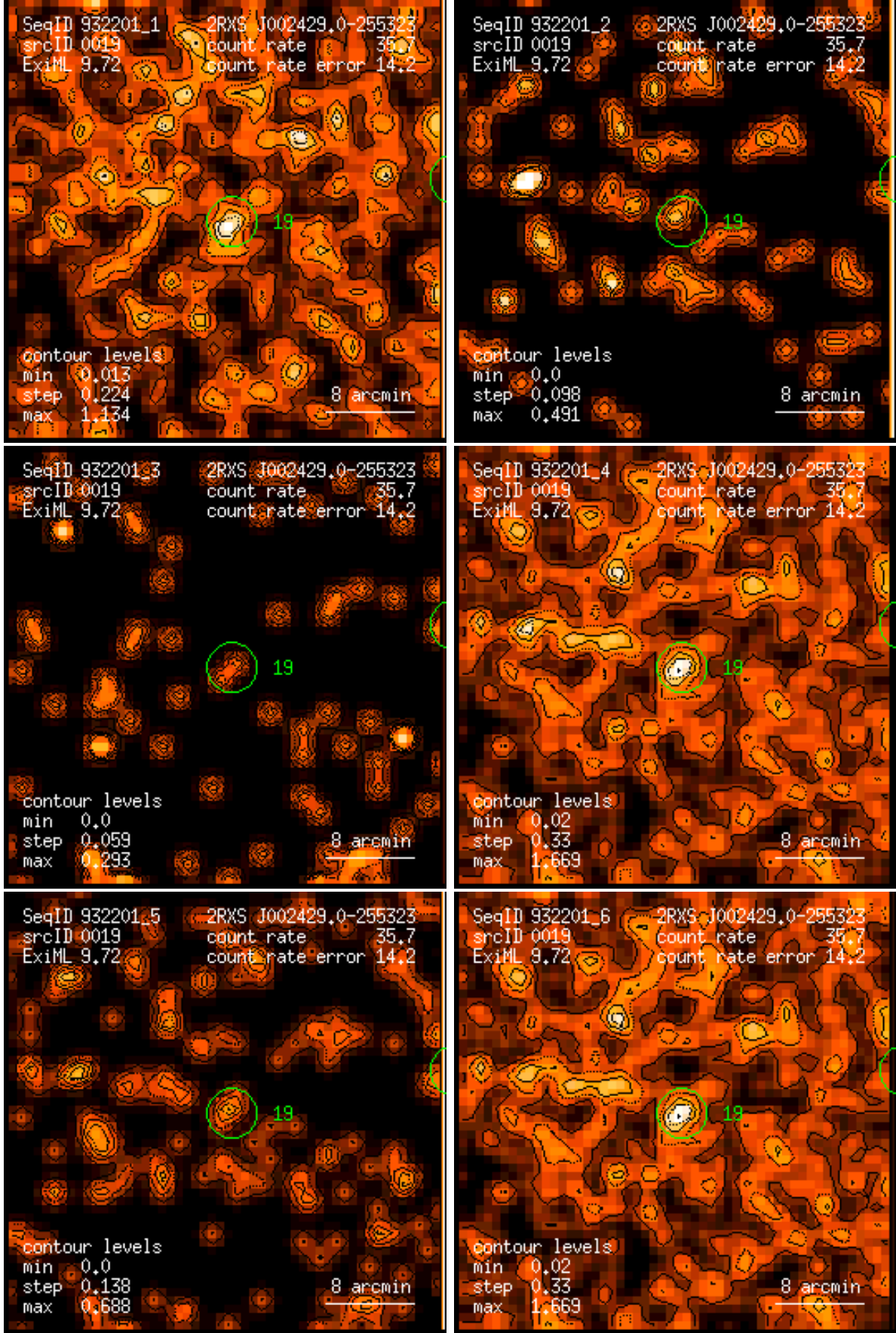
Figure 19: RASS 932201: detection 0019: band rate images, Gaussian filter: (1) PSPC channels 11 – 41, (2) 52 – 90, (3) 91 – 201, (4) 11 – 235, (5) 52 – 201, (6) 11 – 201. Broad band rates in counts/ks. Band rate contour levels in counts/ks/arcmin 2 .
