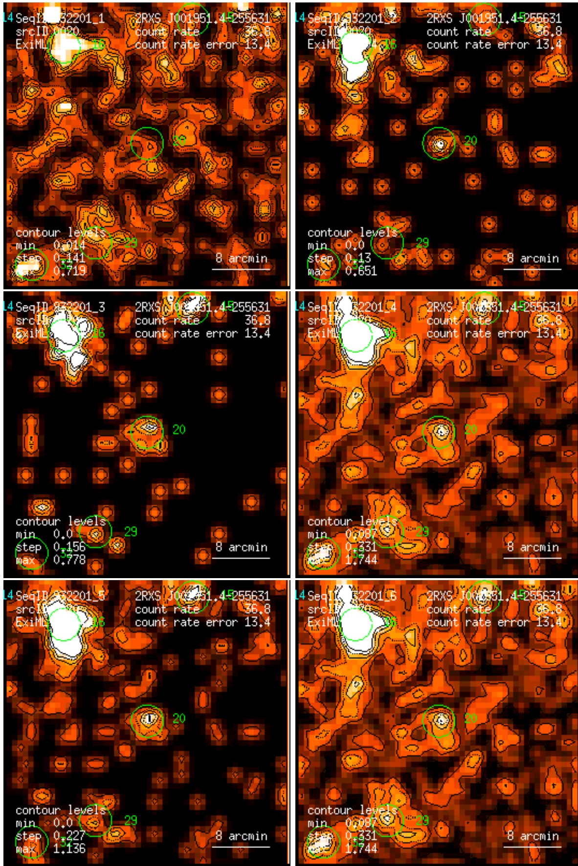
Figure 20: RASS 932201: detection 0020: band rate images, Gaussian filter: (1) PSPC channels 11 – 41, (2) 52 – 90, (3) 91 – 201, (4) 11 – 235, (5) 52 – 201, (6) 11 – 201. Broad band rates in counts/ks. Band rate contour levels in counts/ks/arcmin 2 .
