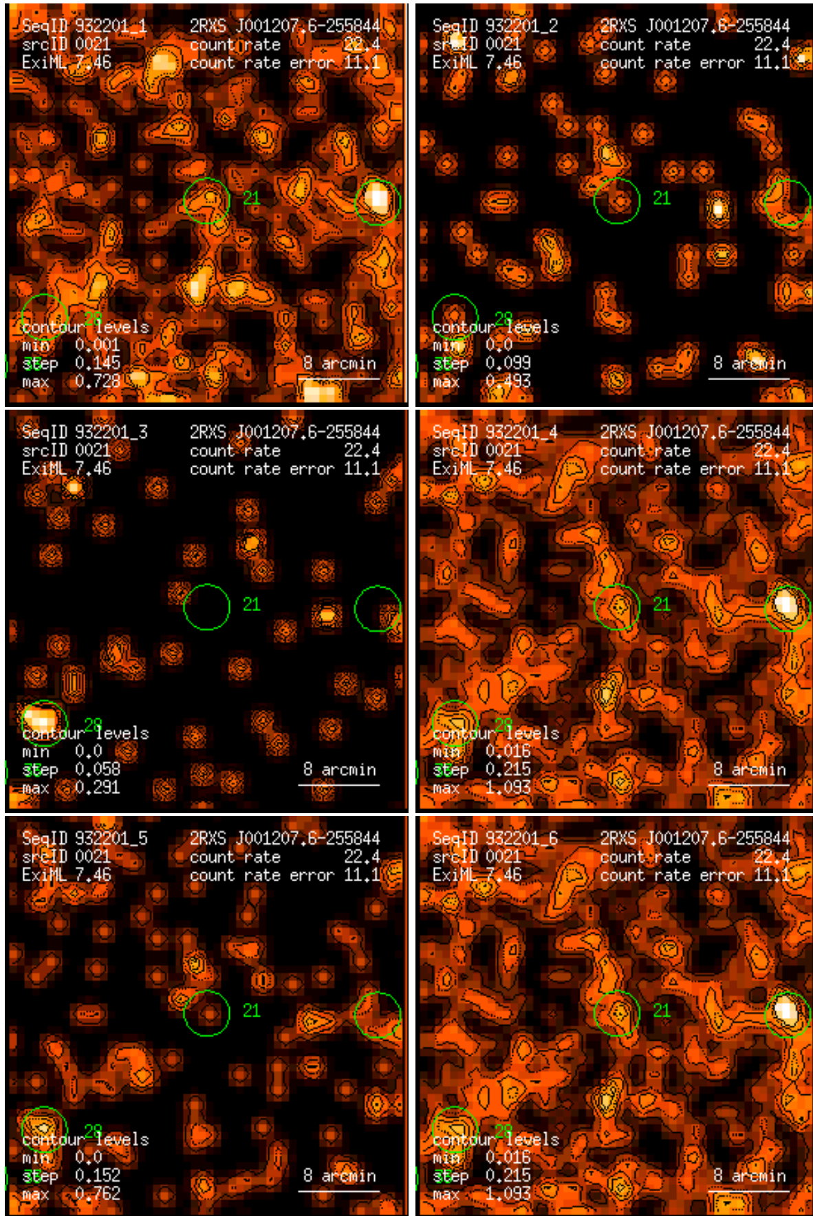
Figure 21: RASS 932201: detection 0021: band rate images, Gaussian filter: (1) PSPC channels 11 – 41, (2) 52 – 90, (3) 91 – 201, (4) 11 – 235, (5) 52 – 201, (6) 11 – 201. Broad band rates in counts/ks. Band rate contour levels in counts/ks/arcmin 2 .
