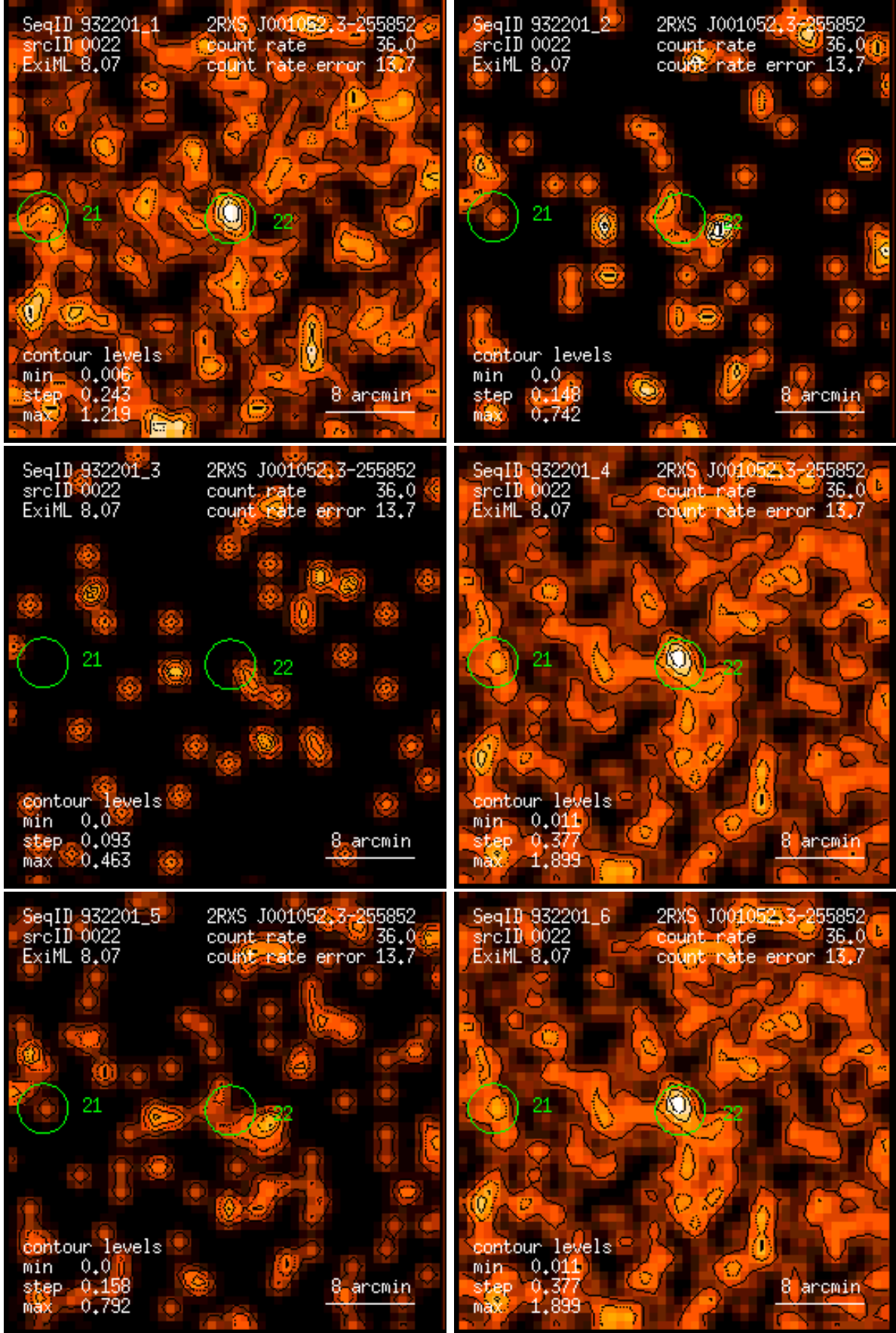
Figure 22: RASS 932201: detection 0022: band rate images, Gaussian filter: (1) PSPC channels 11 – 41, (2) 52 – 90, (3) 91 – 201, (4) 11 – 235, (5) 52 – 201, (6) 11 – 201. Broad band rates in counts/ks. Band rate contour levels in counts/ks/arcmin 2 .
