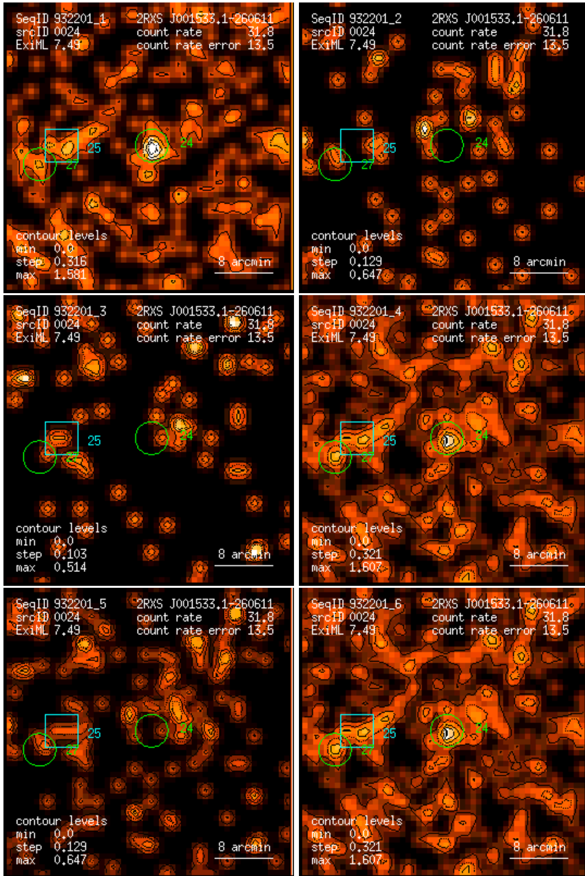
Figure 24: RASS 932201: detection 0024: band rate images, Gaussian filter: (1) PSPC channels 11 – 41, (2) 52 – 90, (3) 91 – 201, (4) 11 – 235, (5) 52 – 201, (6) 11 – 201. Broad band rates in counts/ks. Band rate contour levels in counts/ks/arcmin 2 .
