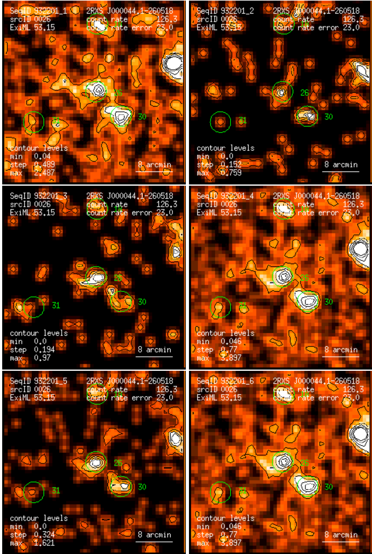
Figure 26: RASS 932201: detection 0026: band rate images, Gaussian filter: (1) PSPC channels 11 – 41, (2) 52 – 90, (3) 91 – 201, (4) 11 – 235, (5) 52 – 201, (6) 11 – 201. Broad band rates in counts/ks. Band rate contour levels in counts/ks/arcmin 2 .
