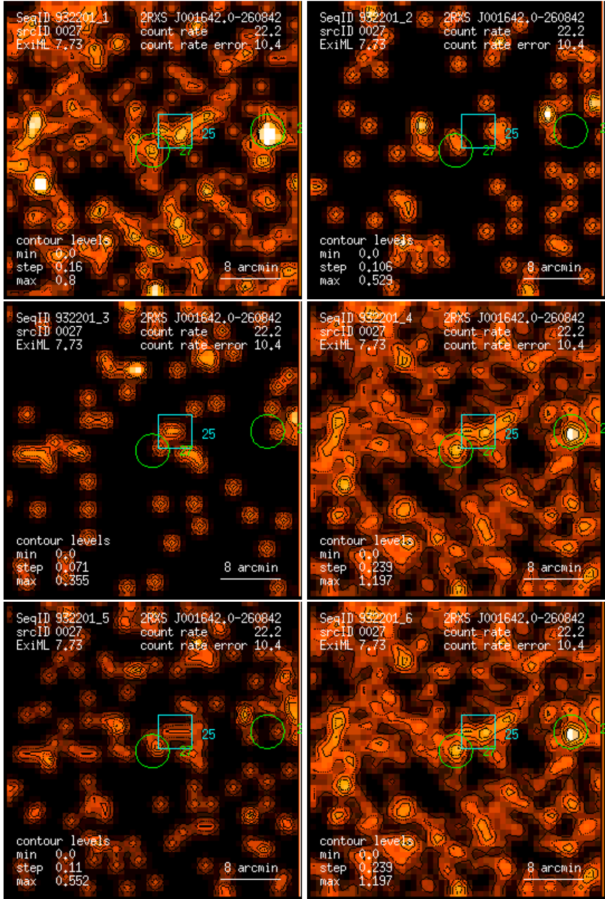
Figure 27: RASS 932201: detection 0027: band rate images, Gaussian filter: (1) PSPC channels 11 – 41, (2) 52 – 90, (3) 91 – 201, (4) 11 – 235, (5) 52 – 201, (6) 11 – 201. Broad band rates in counts/ks. Band rate contour levels in counts/ks/arcmin 2 .
