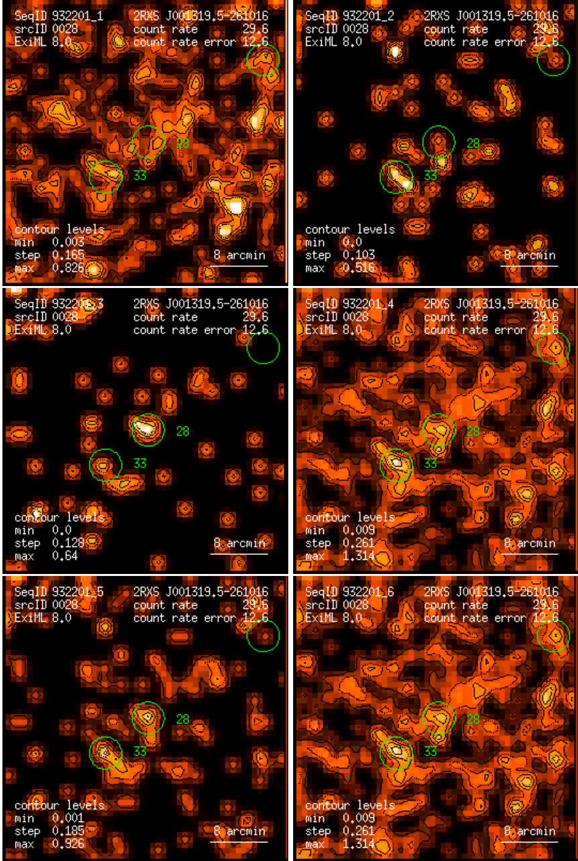
Figure 28: RASS 932201: detection 0028: band rate images, Gaussian filter: (1) PSPC channels 11 – 41, (2) 52 – 90, (3) 91 – 201, (4) 11 – 235, (5) 52 – 201, (6) 11 – 201. Broad band rates in counts/ks. Band rate contour levels in counts/ks/arcmin 2 .
