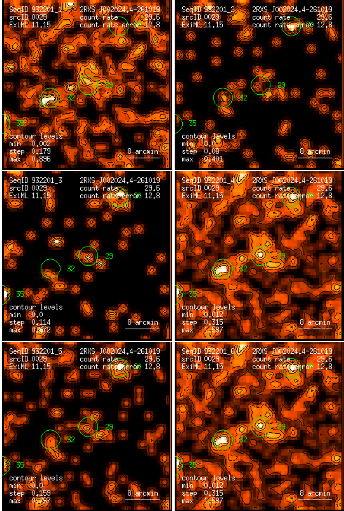
Figure 29: RASS 932201: detection 0029: band rate images, Gaussian filter: (1) PSPC channels 11 – 41, (2) 52 – 90, (3) 91 – 201, (4) 11 – 235, (5) 52 – 201, (6) 11 – 201. Broad band rates in counts/ks. Band rate contour levels in counts/ks/arcmin 2 .
