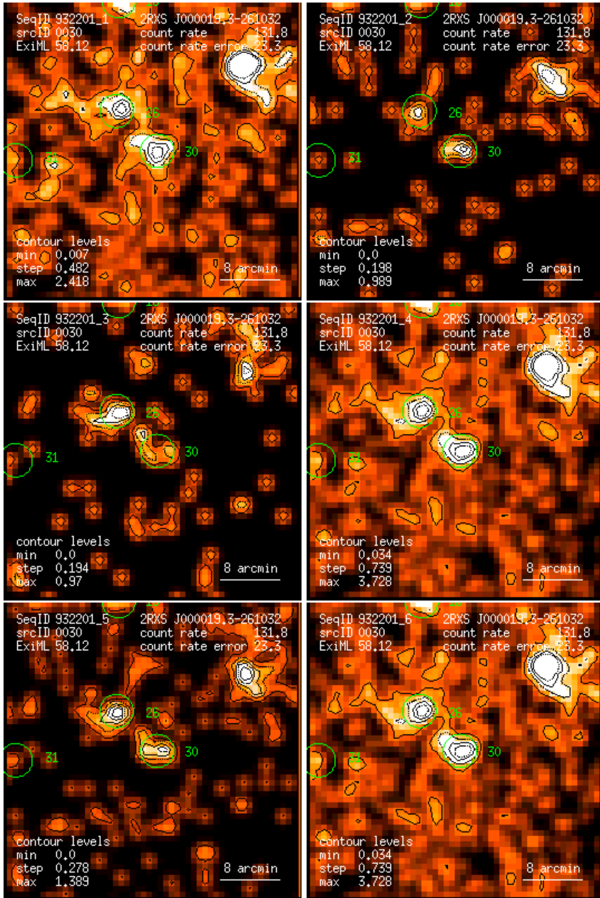
Figure 30: RASS 932201: detection 0030: band rate images, Gaussian filter: (1) PSPC channels 11 – 41, (2) 52 – 90, (3) 91 – 201, (4) 11 – 235, (5) 52 – 201, (6) 11 – 201. Broad band rates in counts/ks. Band rate contour levels in counts/ks/arcmin 2 .
