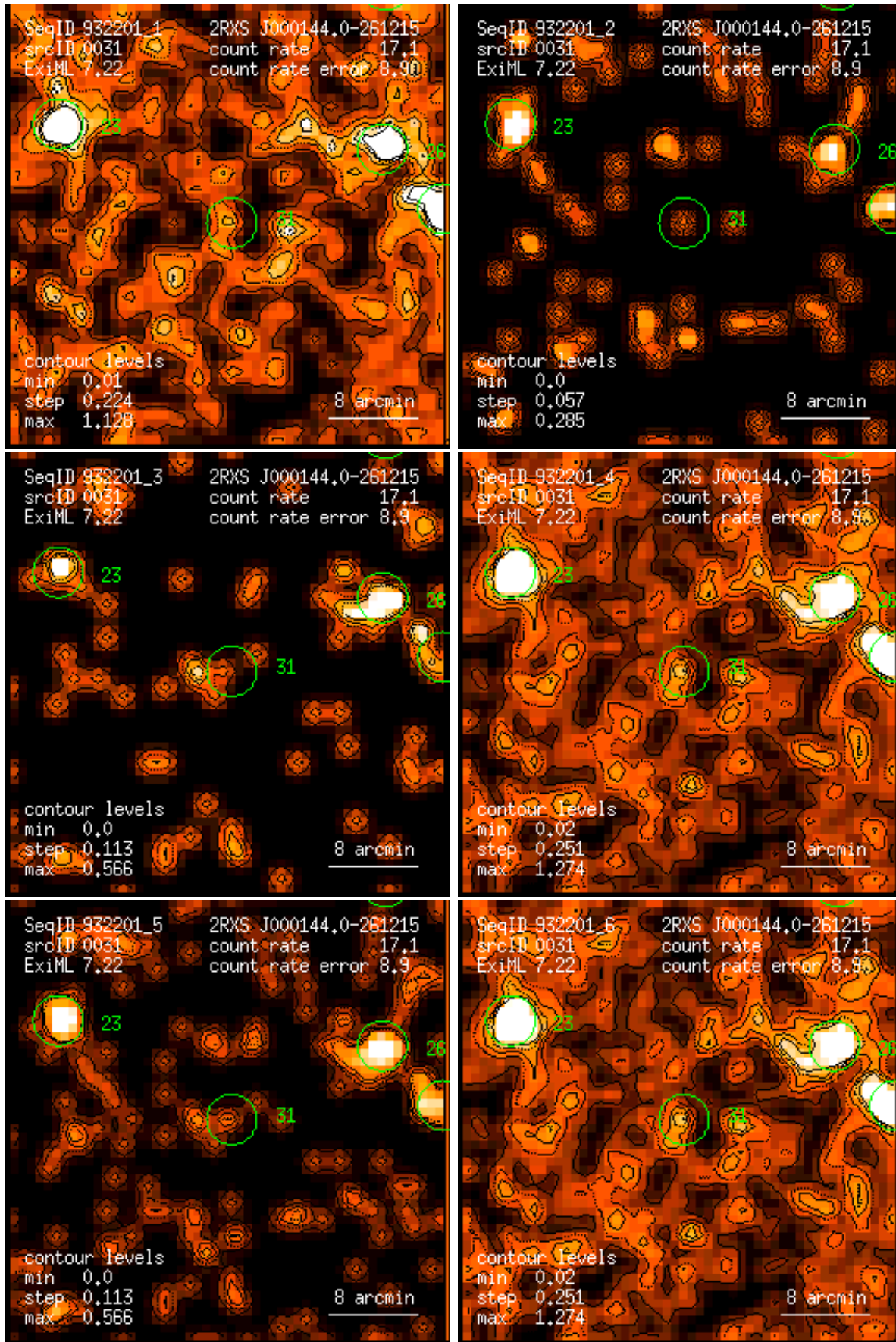
Figure 31: RASS 932201: detection 0031: band rate images, Gaussian filter: (1) PSPC channels 11 – 41, (2) 52 – 90, (3) 91 – 201, (4) 11 – 235, (5) 52 – 201, (6) 11 – 201. Broad band rates in counts/ks. Band rate contour levels in counts/ks/arcmin 2 .
