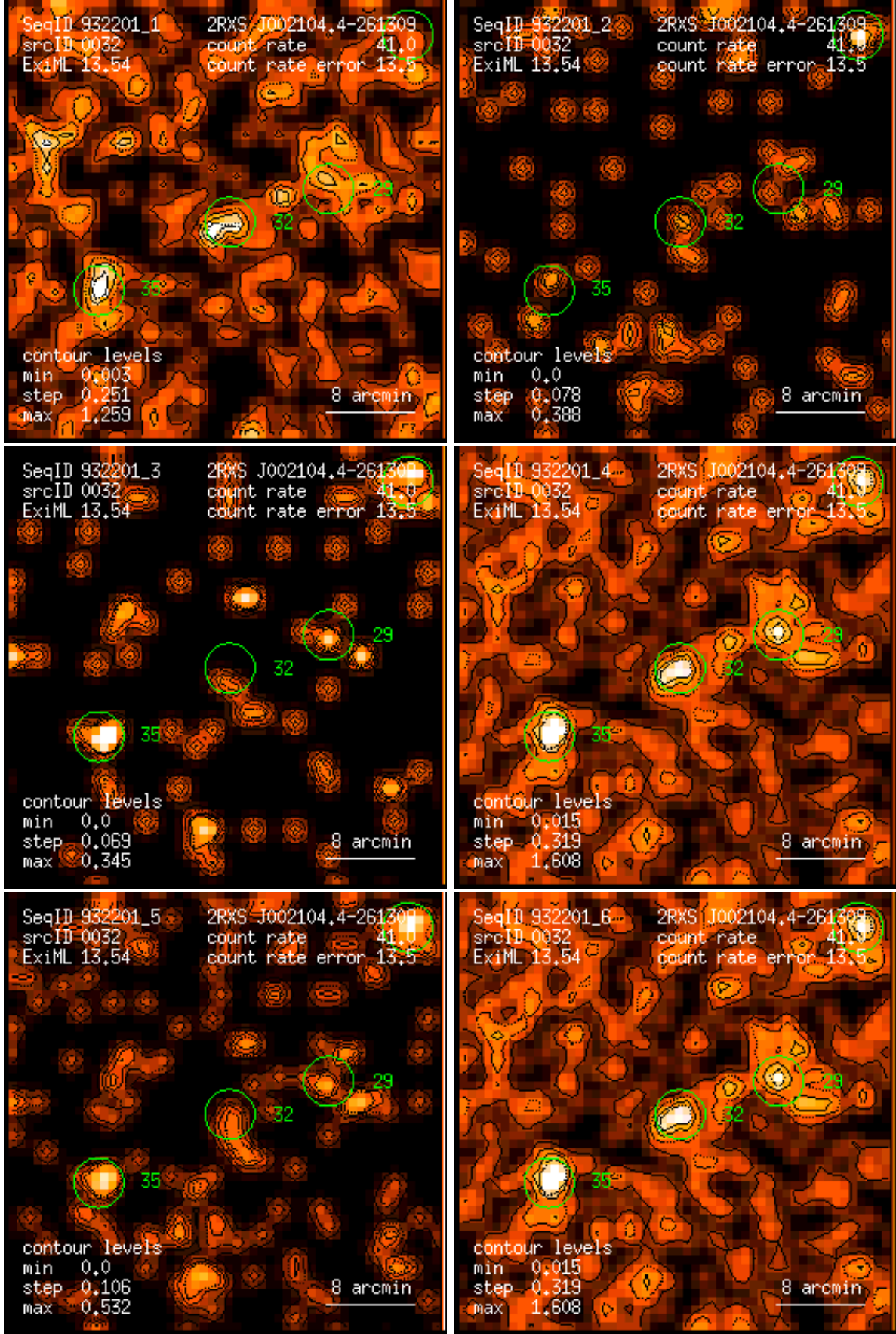
Figure 32: RASS 932201: detection 0032: band rate images, Gaussian filter: (1) PSPC channels 11 – 41, (2) 52 – 90, (3) 91 – 201, (4) 11 – 235, (5) 52 – 201, (6) 11 – 201. Broad band rates in counts/ks. Band rate contour levels in counts/ks/arcmin 2 .
