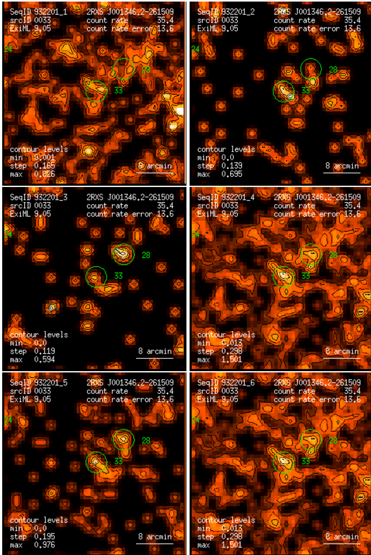
Figure 33: RASS 932201: detection 0033: band rate images, Gaussian filter: (1) PSPC channels 11 – 41, (2) 52 – 90, (3) 91 – 201, (4) 11 – 235, (5) 52 – 201, (6) 11 – 201. Broad band rates in counts/ks. Band rate contour levels in counts/ks/arcmin 2 .
