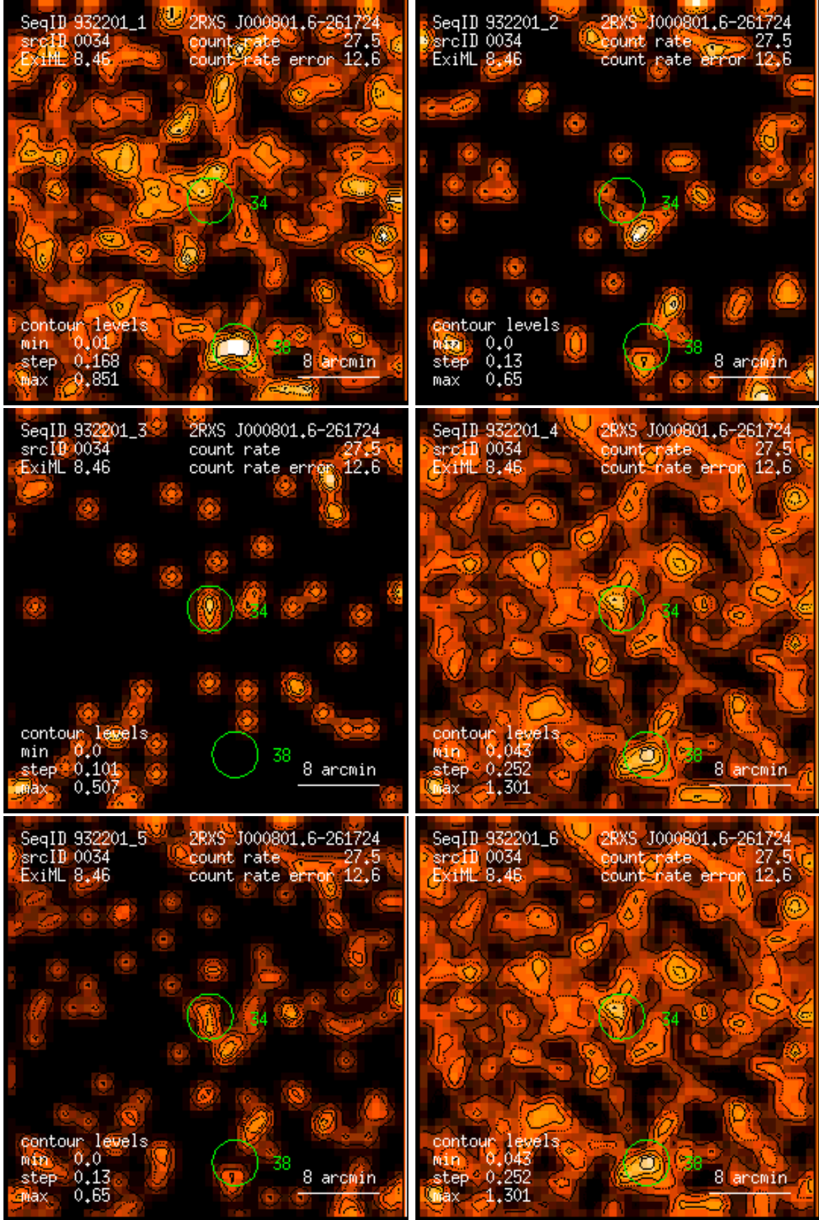
Figure 34: RASS 932201: detection 0034: band rate images, Gaussian filter: (1) PSPC channels 11 – 41, (2) 52 – 90, (3) 91 – 201, (4) 11 – 235, (5) 52 – 201, (6) 11 – 201. Broad band rates in counts/ks. Band rate contour levels in counts/ks/arcmin 2 .
