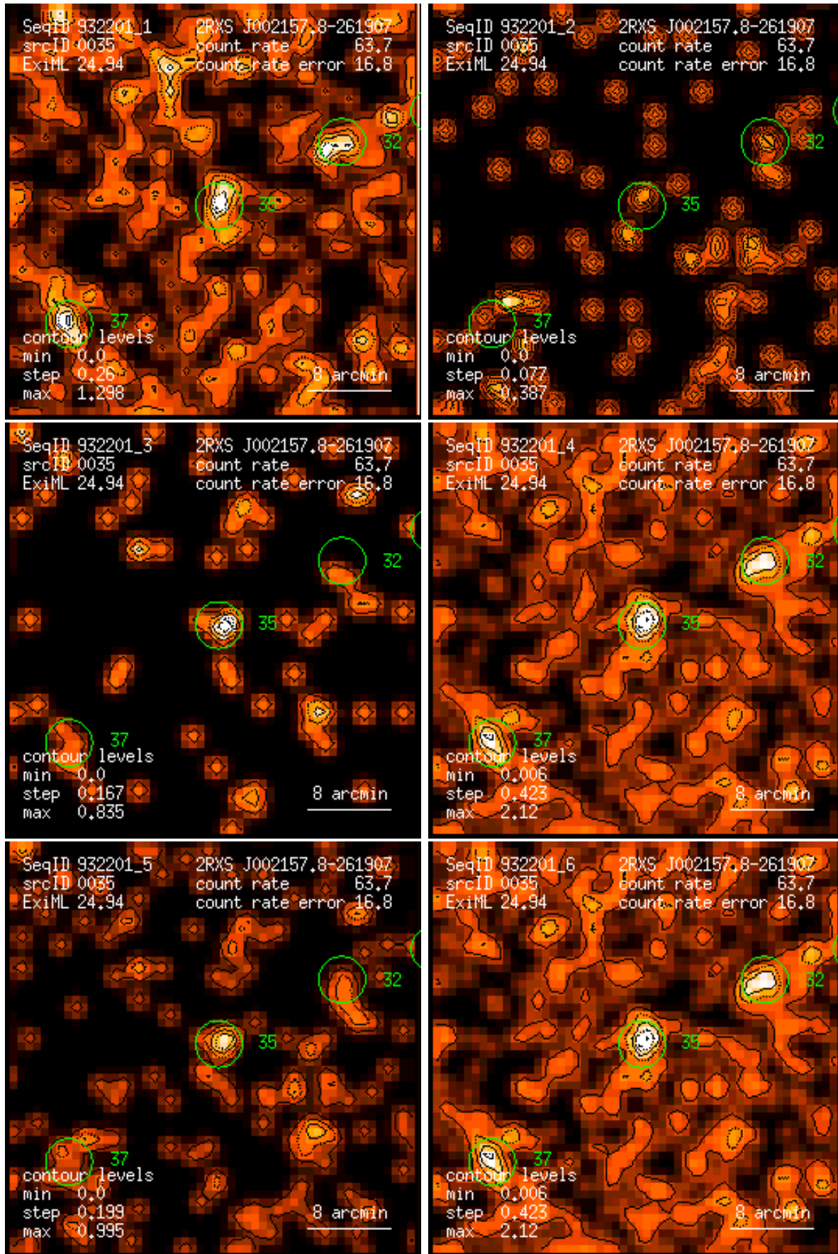
Figure 35: RASS 932201: detection 0035: band rate images, Gaussian filter: (1) PSPC channels 11 – 41, (2) 52 – 90, (3) 91 – 201, (4) 11 – 235, (5) 52 – 201, (6) 11 – 201. Broad band rates in counts/ks. Band rate contour levels in counts/ks/arcmin 2 .
