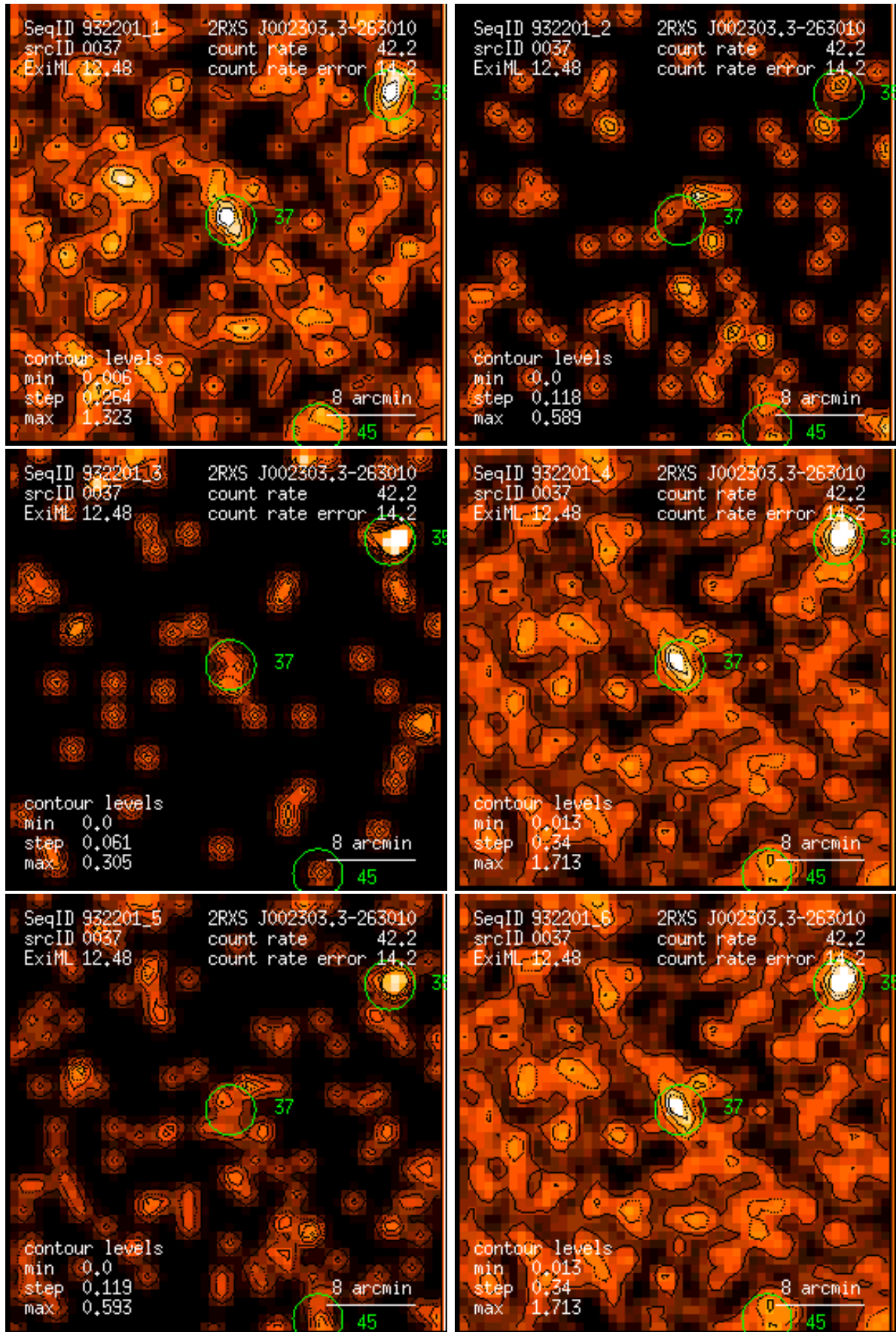
Figure 37: RASS 932201: detection 0037: band rate images, Gaussian filter: (1) PSPC channels 11 – 41, (2) 52 – 90, (3) 91 – 201, (4) 11 – 235, (5) 52 – 201, (6) 11 – 201. Broad band rates in counts/ks. Band rate contour levels in counts/ks/arcmin 2 .
