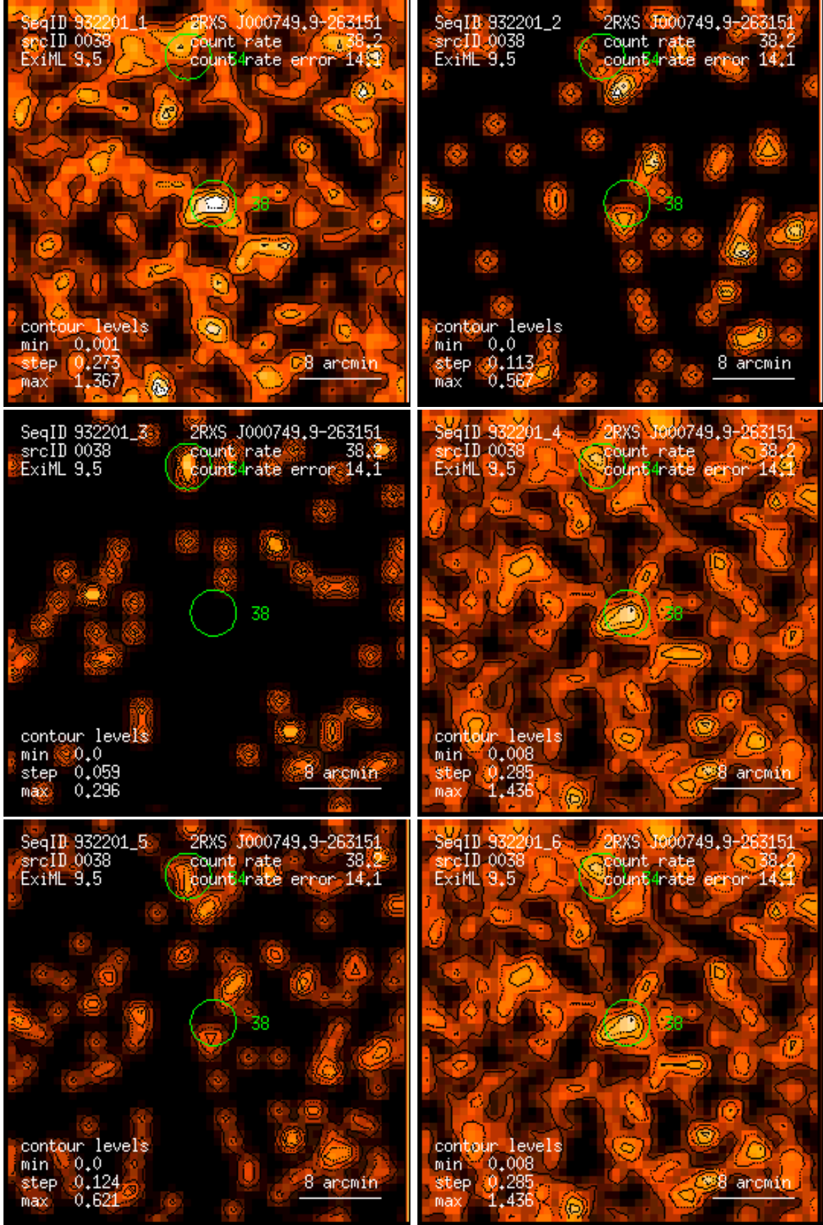
Figure 38: RASS 932201: detection 0038: band rate images, Gaussian filter: (1) PSPC channels 11 – 41, (2) 52 – 90, (3) 91 – 201, (4) 11 – 235, (5) 52 – 201, (6) 11 – 201. Broad band rates in counts/ks. Band rate contour levels in counts/ks/arcmin 2 .
