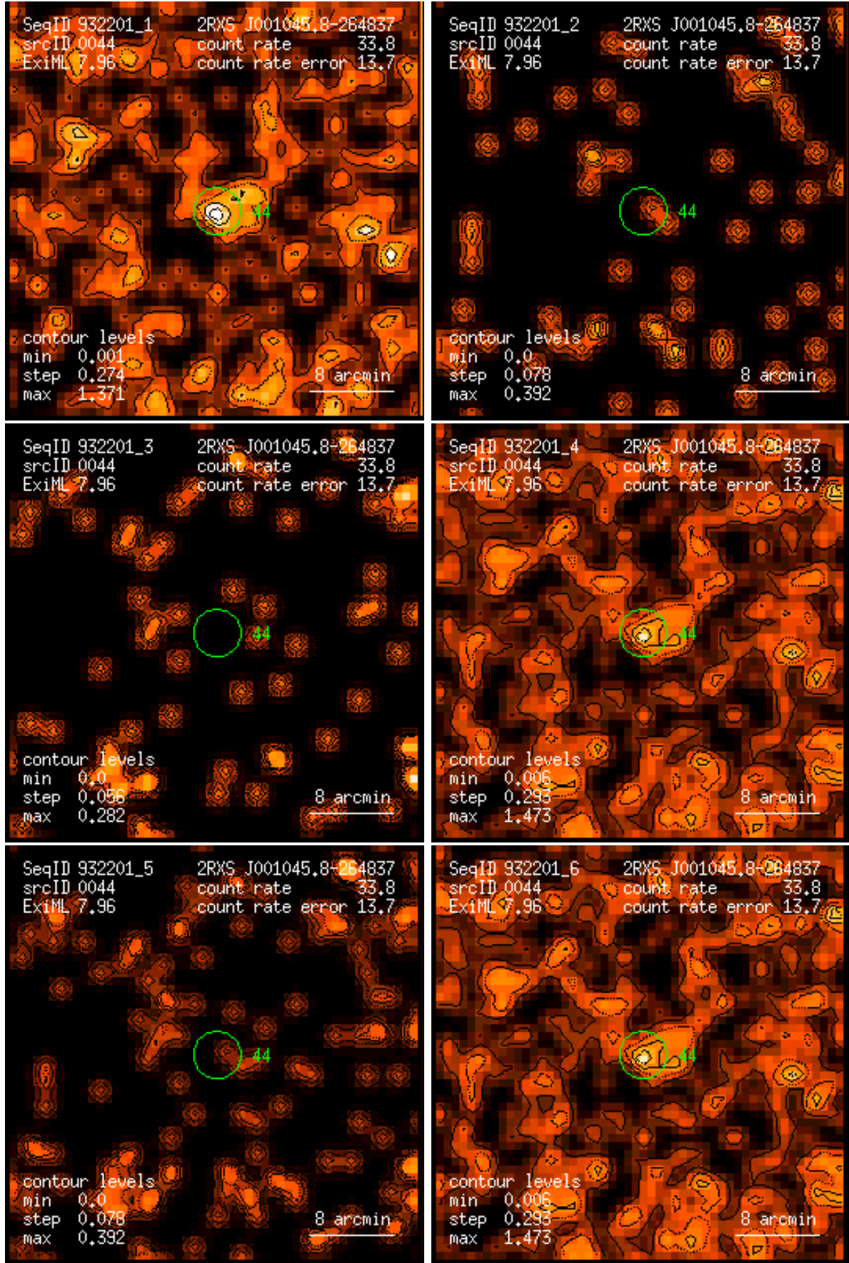
Figure 44: RASS 932201: detection 0044: band rate images, Gaussian filter: (1) PSPC channels 11 – 41, (2) 52 – 90, (3) 91 – 201, (4) 11 – 235, (5) 52 – 201, (6) 11 – 201. Broad band rates in counts/ks. Band rate contour levels in counts/ks/arcmin 2 .
