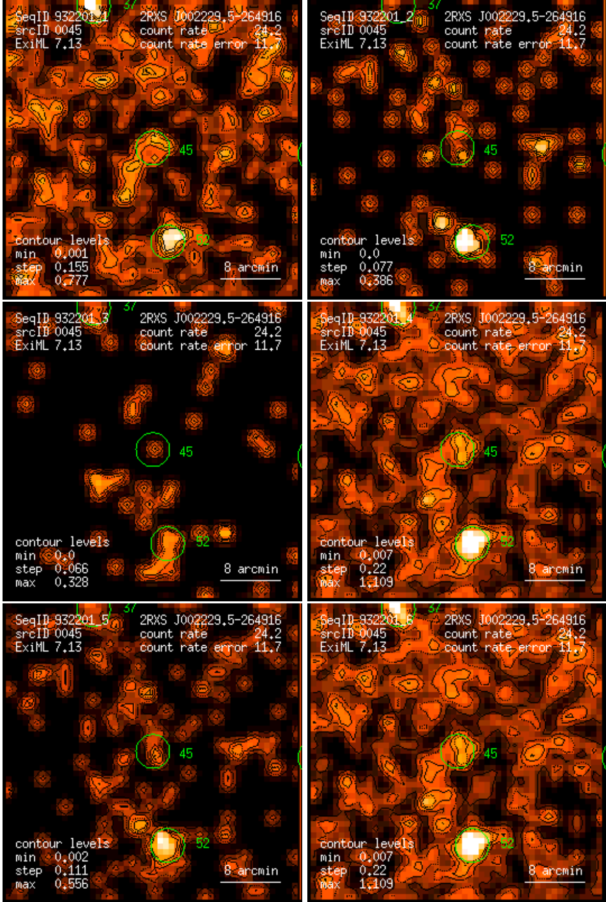
Figure 45: RASS 932201: detection 0045: band rate images, Gaussian filter: (1) PSPC channels 11 – 41, (2) 52 – 90, (3) 91 – 201, (4) 11 – 235, (5) 52 – 201, (6) 11 – 201. Broad band rates in counts/ks. Band rate contour levels in counts/ks/arcmin 2 .
